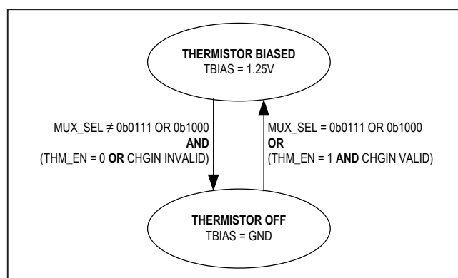
Figure 11. Thermistor Bias State Diagram
