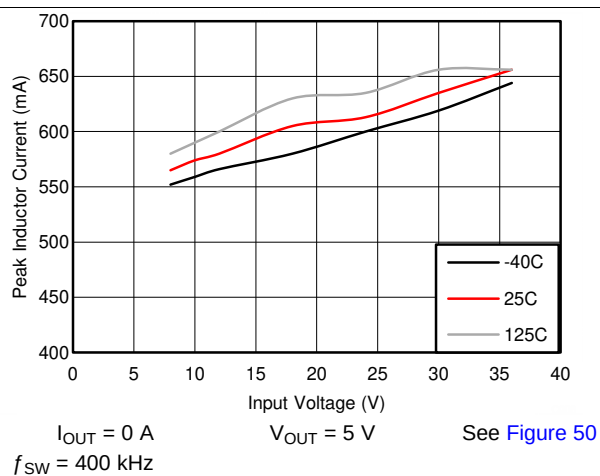
Figure 6. I_{PEAK-MIN}
