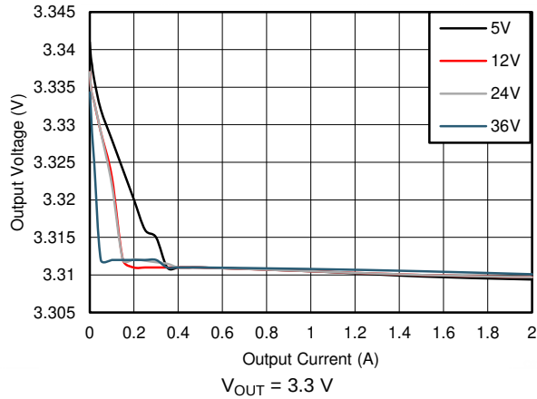
Figure 44. Line and Load Regulation
