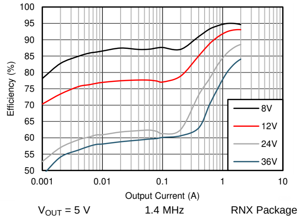
Figure 34. Efficiency
