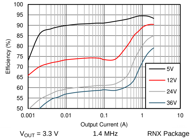
Figure 35. Efficiency
