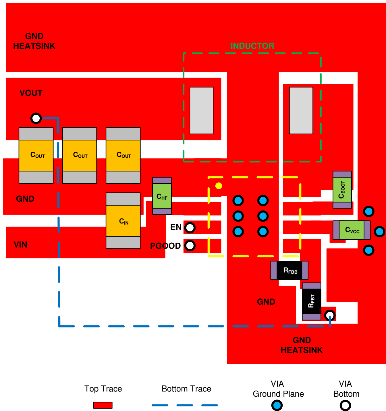
Figure 52. Example Layout for HSOIC (DDA) Package
