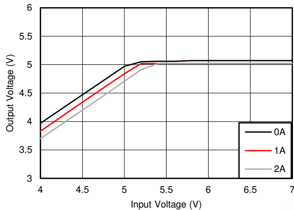
Figure 15. Overall Dropout Characteristic V_{OUT} = 5\text{ V}
