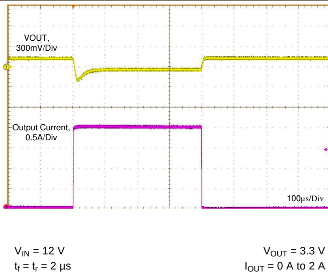
Figure 48. Load Transient
