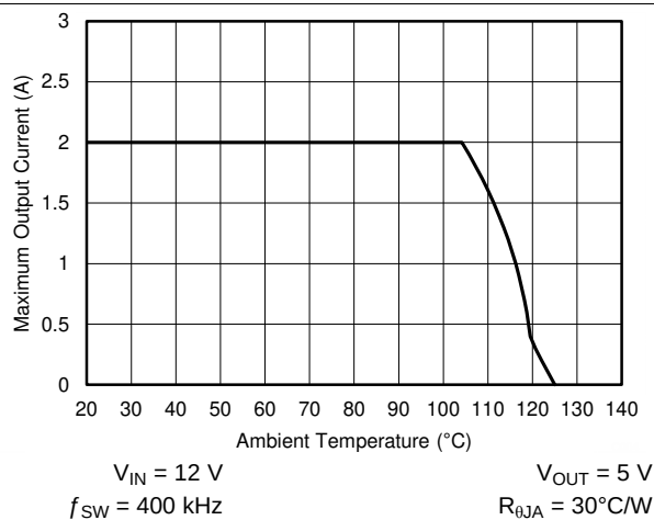
Figure 24. Maximum Output Current versus Ambient Temperature
