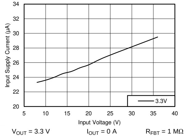
Figure 45. Input Supply Current
