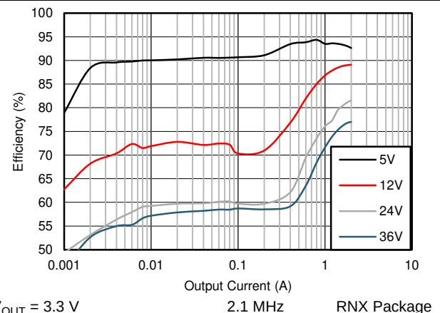
Figure 37. Efficiency
