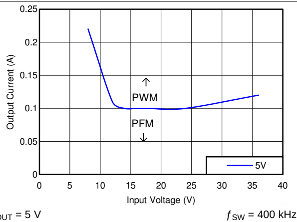
Figure 40. Mode Change Thresholds
