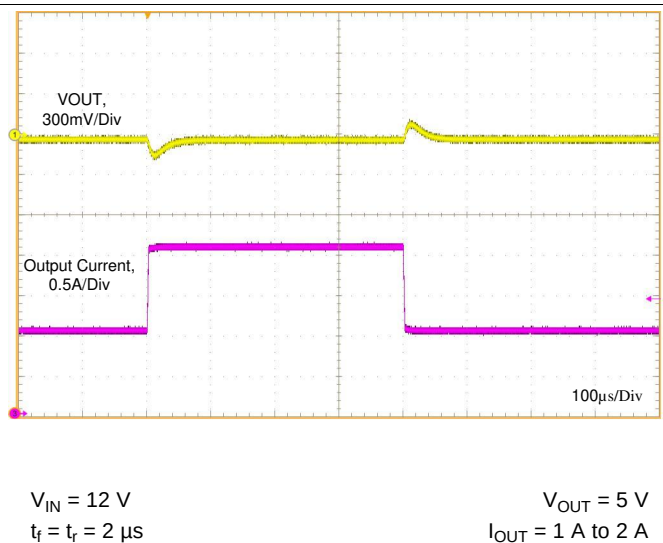
Figure 43. Load Transient
