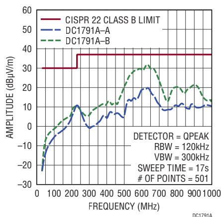
Figure 1. DC1791A Radiated Emissions
