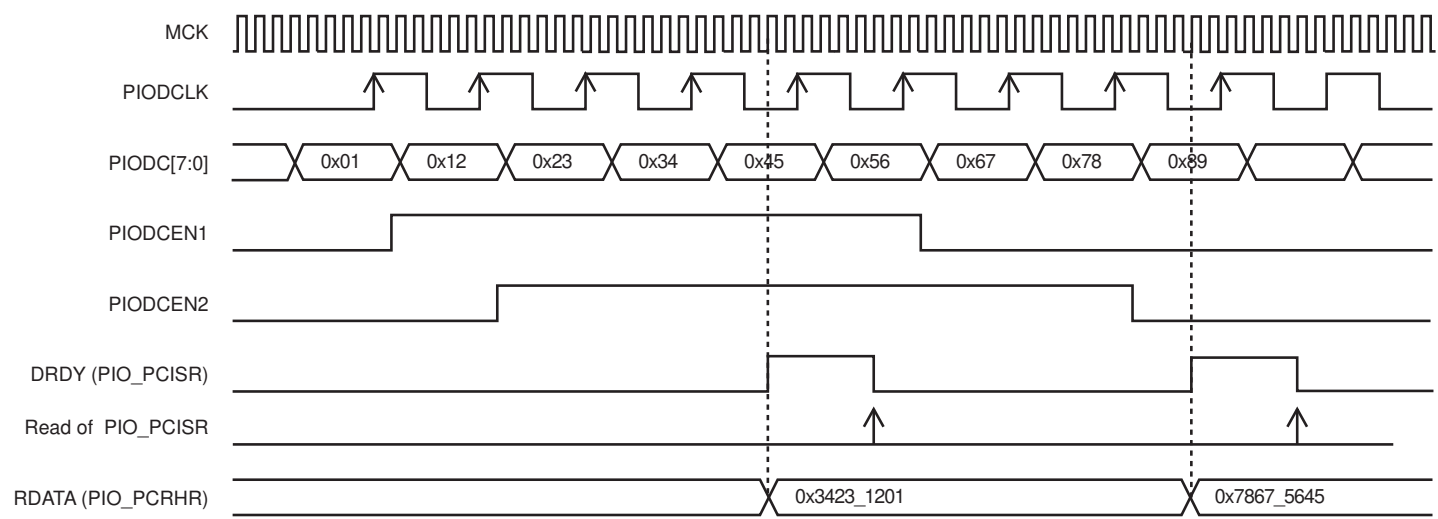
Figure 31-10. Parallel Capture Mode Waveforms (DSIZE = 2, ALWYS = 1, HALFS = 0)
