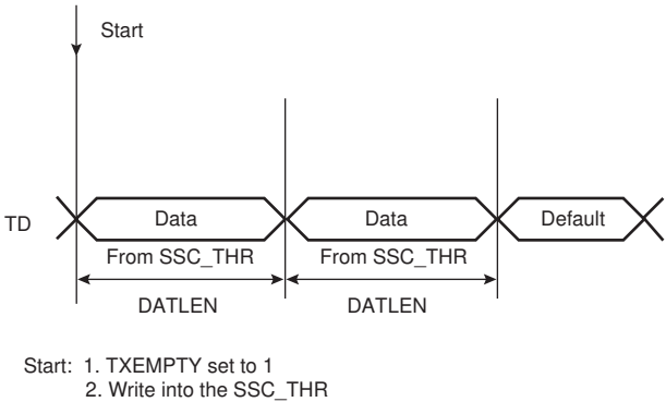
Figure 32-17. Transmit Frame Format in Continuous Mode (STTDLY = 0)
