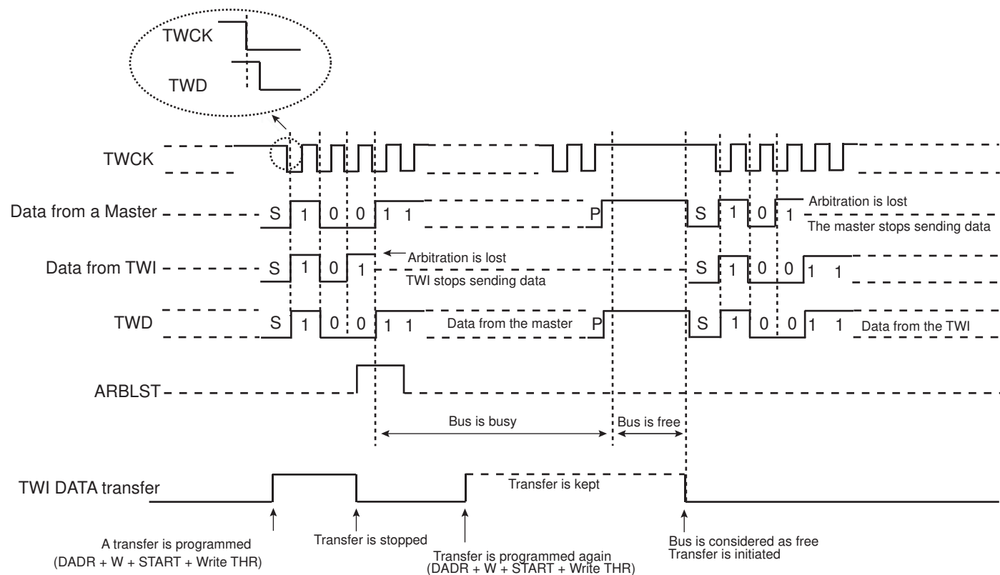
Figure 34-21. Arbitration Cases
