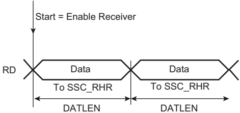
Figure 32-18. Receive Frame Format in Continuous Mode (STTDLY = 0)
