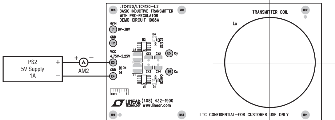
Figure 7b. Using the V_{CC} Input
