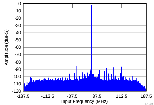
Figure 70. FFT in 8X Decimation (Complex Output)
