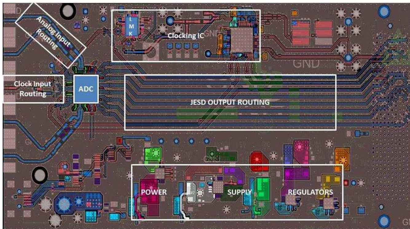
Figure 266. ADC32RF8xEVM Layout
