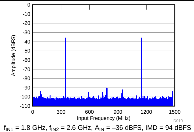
Figure 24. FFT for Two-Tone Input Signal (–36 dBFS, f_s = 2457.6 \text{ MSPS} )
