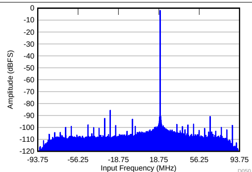
Figure 72. FFT in 10X Decimation (Complex Output)
