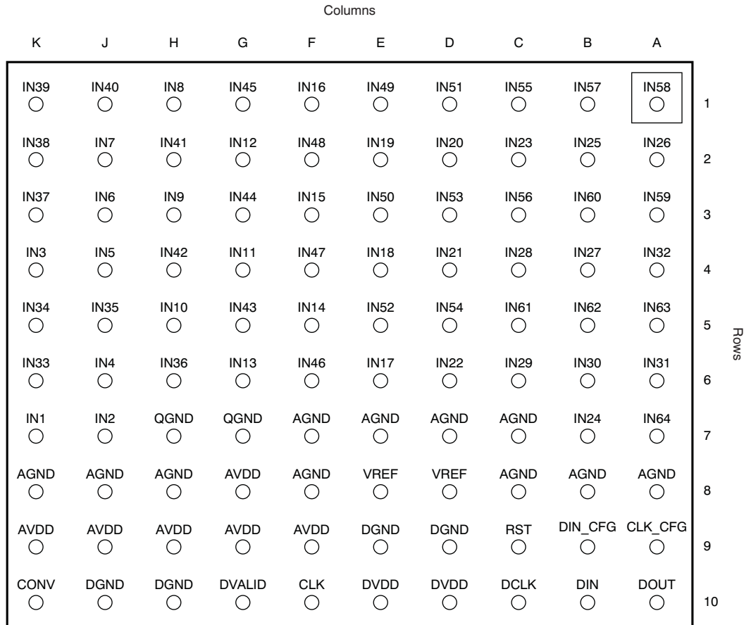
Pin Functions
