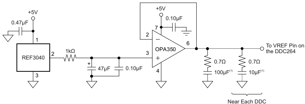
Figure 32. Recommended External Voltage Reference Circuit for Best Low-Noise Operation
