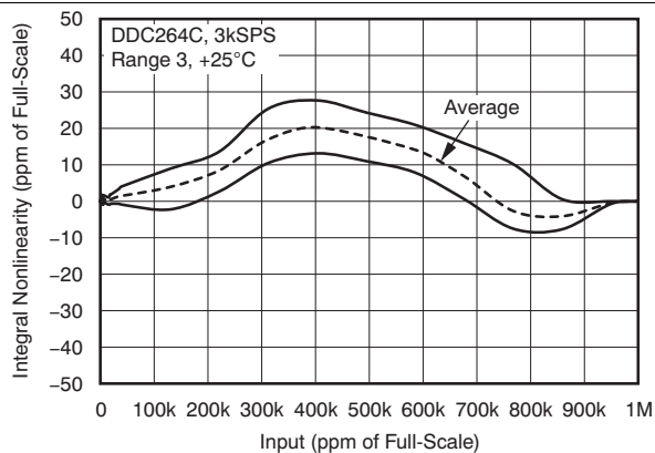
Figure 1. Integral Nonlinearity
