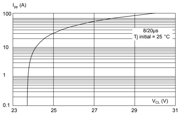
Figure 4. Peak pulse current versus clamping voltage (max value, 8/20 μs)
