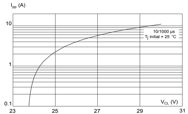
Figure 5. Peak pulse current versus clamping voltage (max value, 10/1000 μs)
