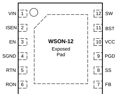
Figure 4. WSO-12 Top View
