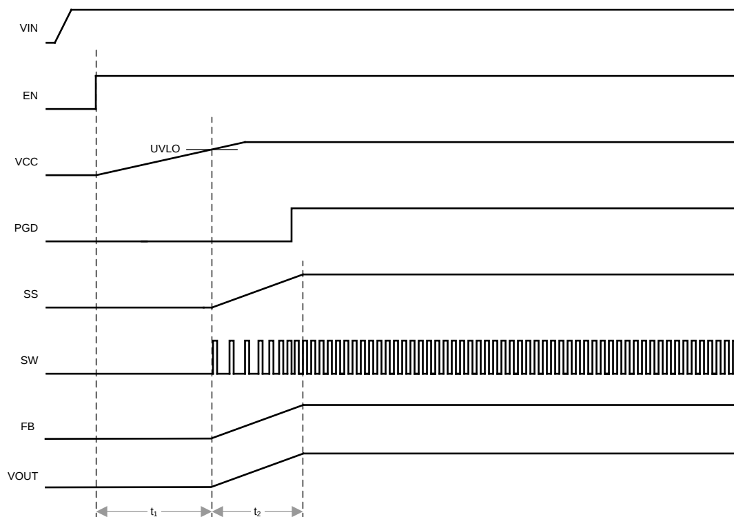
Figure 6. Start-Up Sequence
