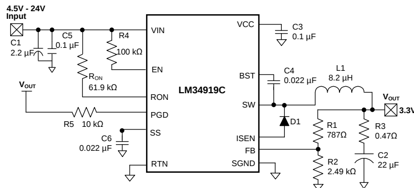
Figure 9. Example Circuit
