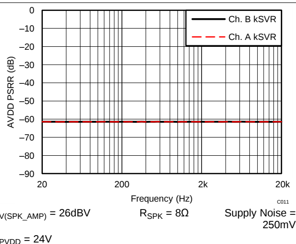
Figure 41. AVDD PSRR vs Frequency - BTL
