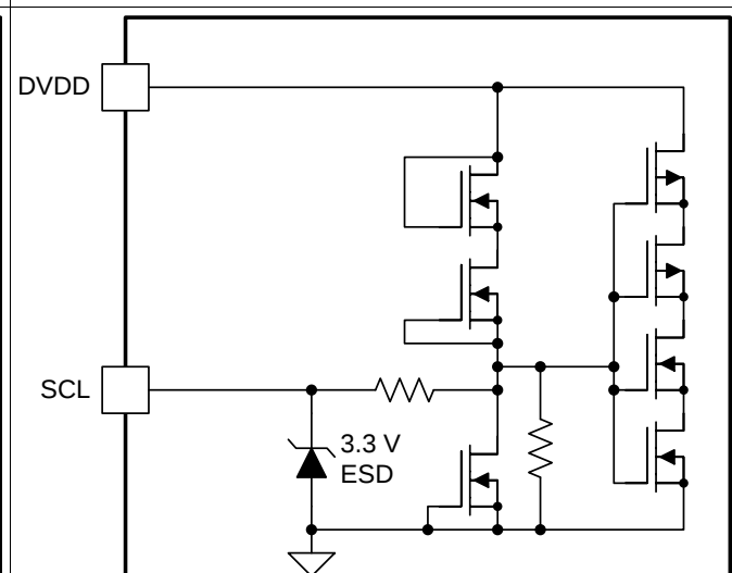
Figure 12. SCL Pin
