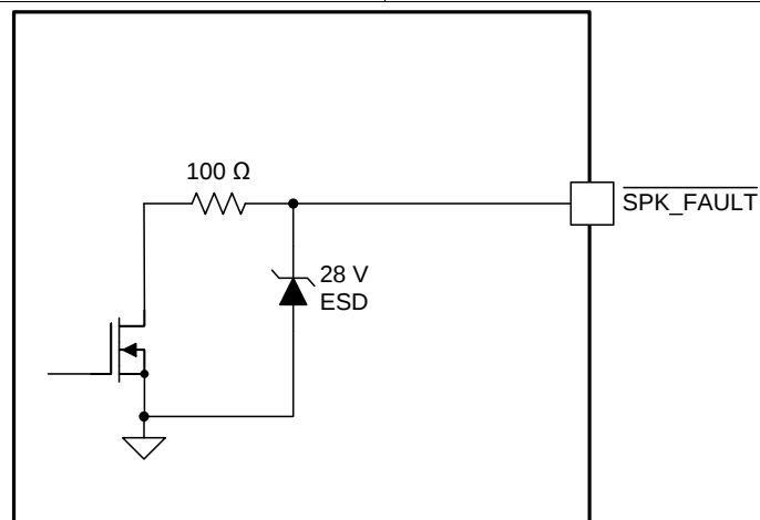
Figure 19. SPK_FAULT Pin
