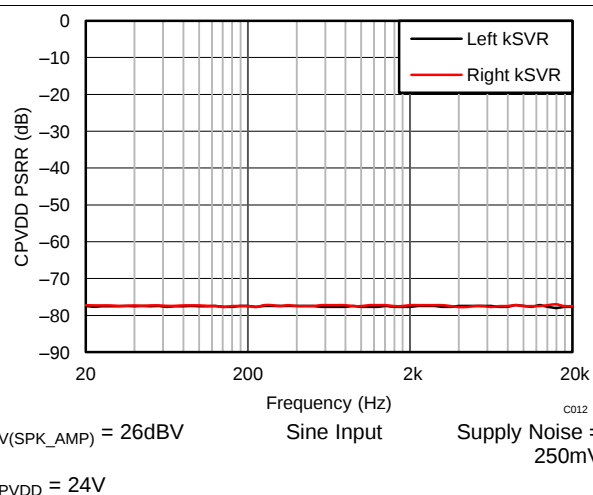
Figure 42. CPVDD PSRR vs Frequency - BTL
