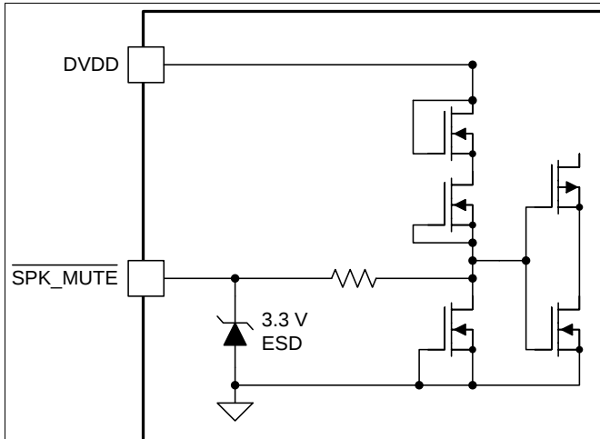
Figure 15. SPK_MUTE Pin
