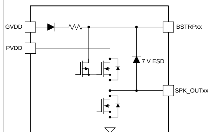
Figure 5. BSTRPxx Pins
