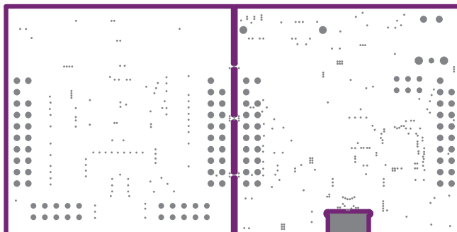
Figure 35. TPS65981EVM GND Plane 3
