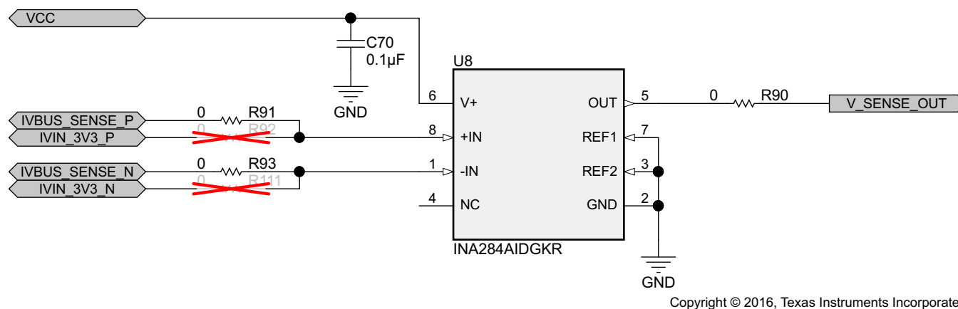
Figure 22. Current-Sense Block
