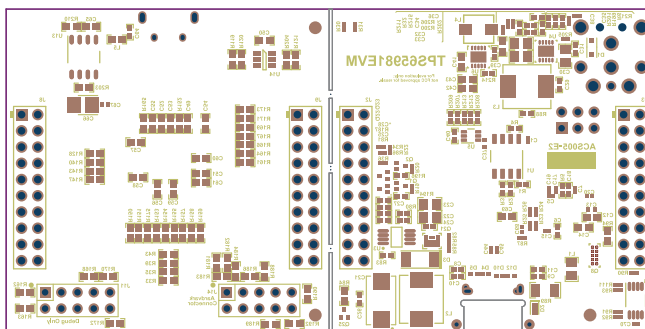
Figure 37. TPS65981EVM Bottom Layer Component View
