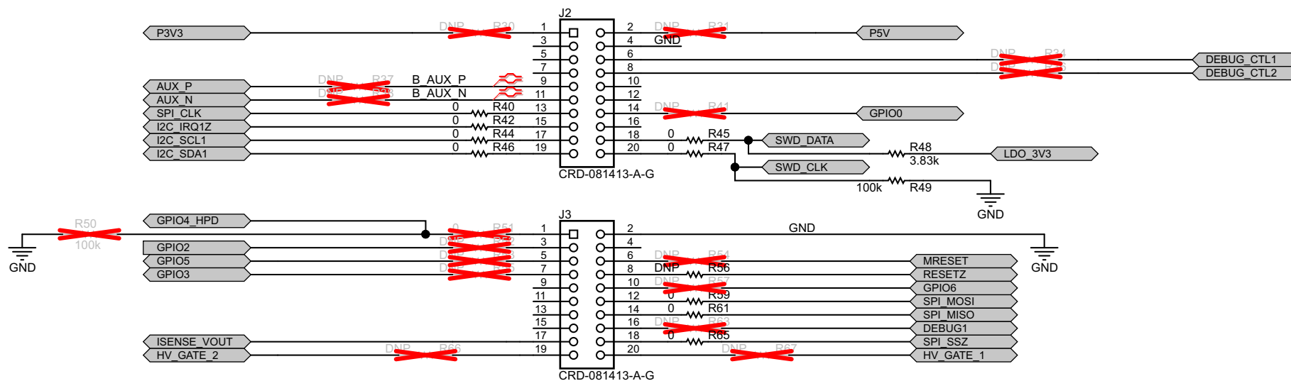
Figure 27. TPS65981EVM Debug Connector Block
