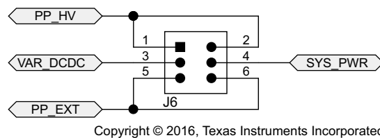
Figure 21. Power Jumper Block
