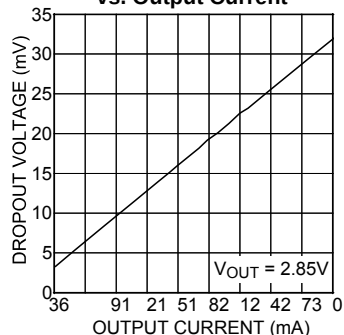
LDO2 Dropout Voltage vs. Output Current
