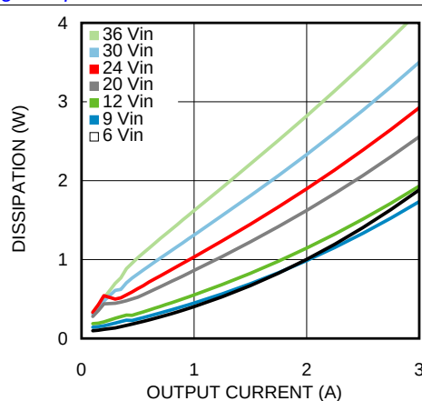
Figure 26. Dissipation 2.5-V Output at 85°C Ambient
