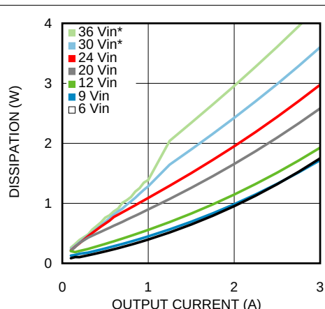
Figure 28. Dissipation 1.8-V Output at 85°C Ambient
