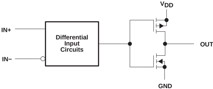
functional block diagram (each comparator)
