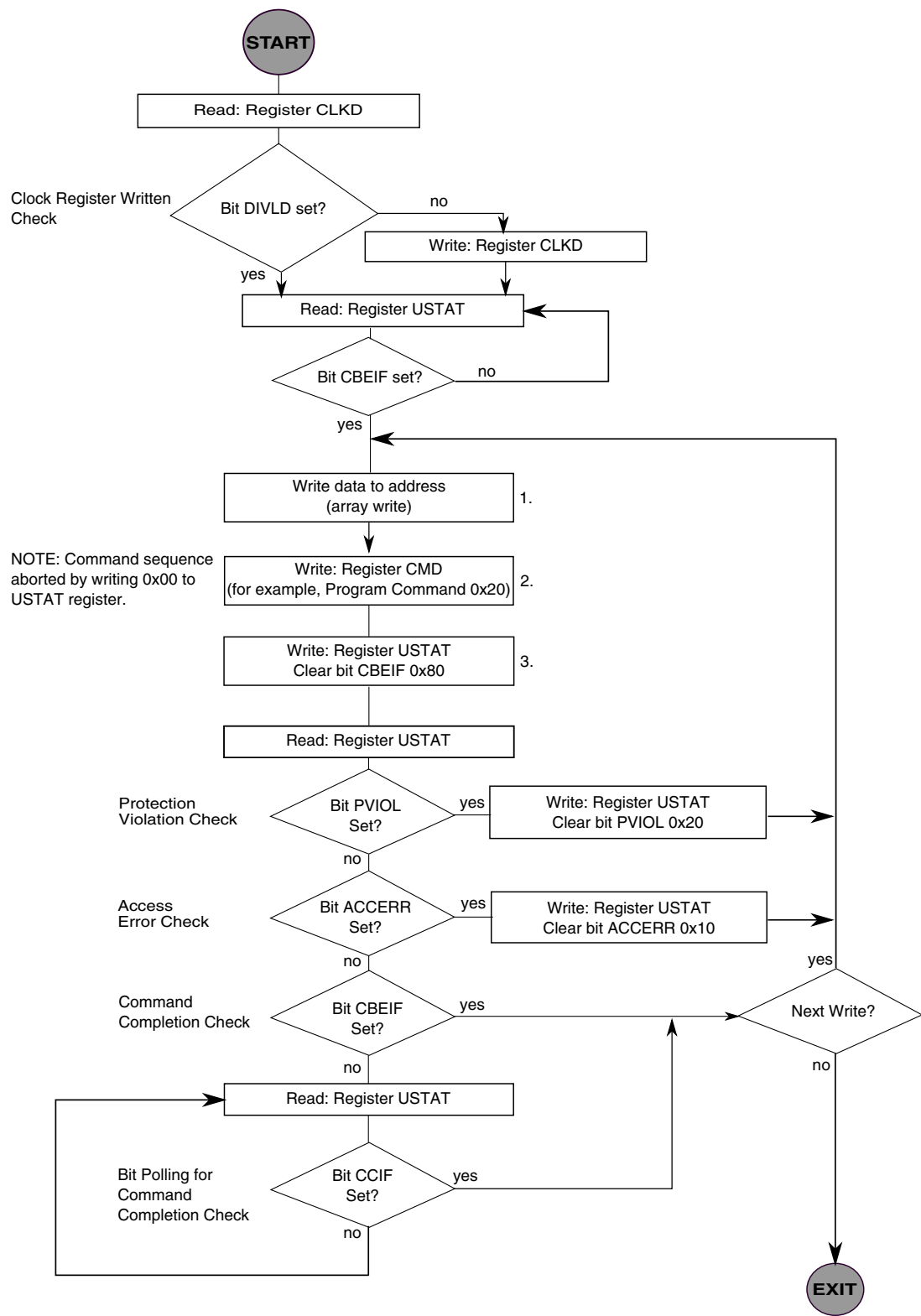
Figure 20-13. Command Sequence Flow Chart
