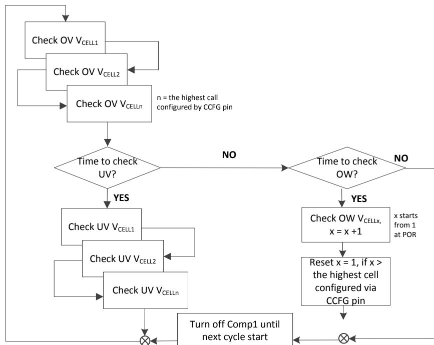
Figure 8. Comparator 1 Flowchart
