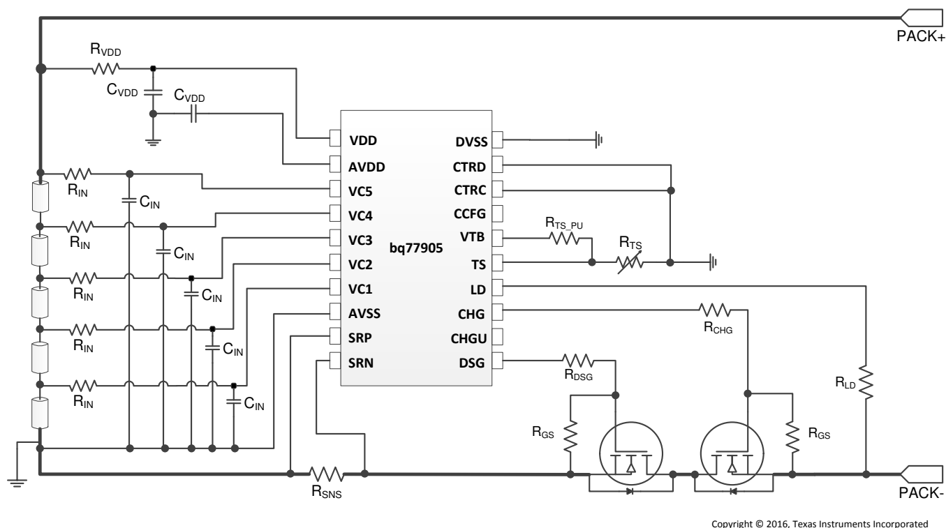
Figure 33. BQ77905 with Five Cells
