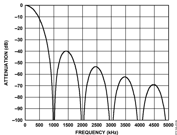
Figure 21. Typical Digital Filter Response at f_{ADC} = 1 kHz (ADCFLT = 0x0007)
