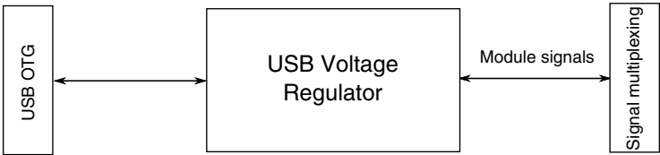
Figure 3-53. USB Voltage Regulator configuration
