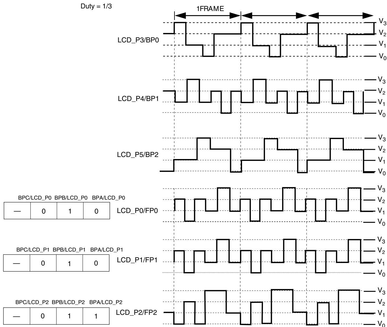
Figure 52-40. LCD waveforms
