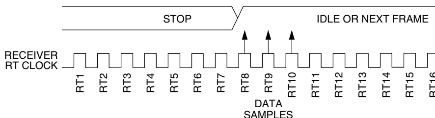
Figure 48-299. Fast data
