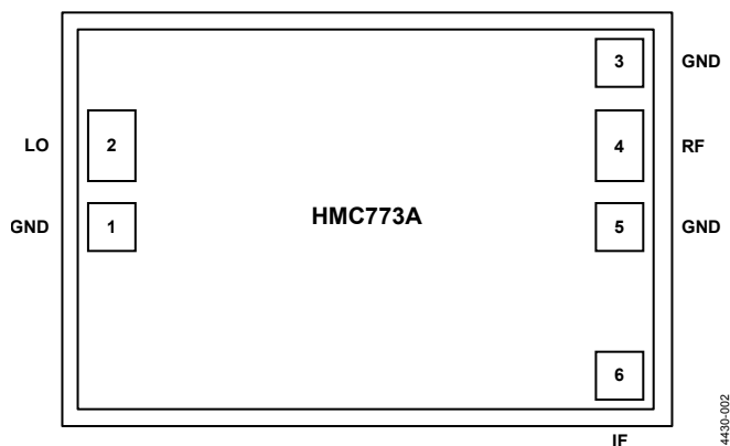
Figure 2. Pin Configuration
