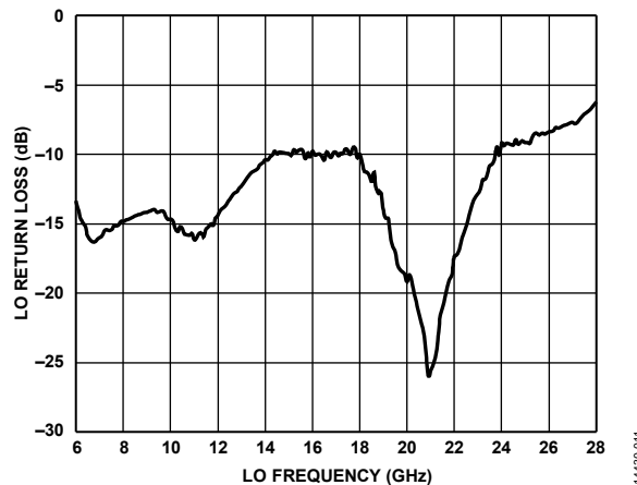
Figure 11. LO Return Loss vs. LO Frequency, LO Drive = 13 dBm
