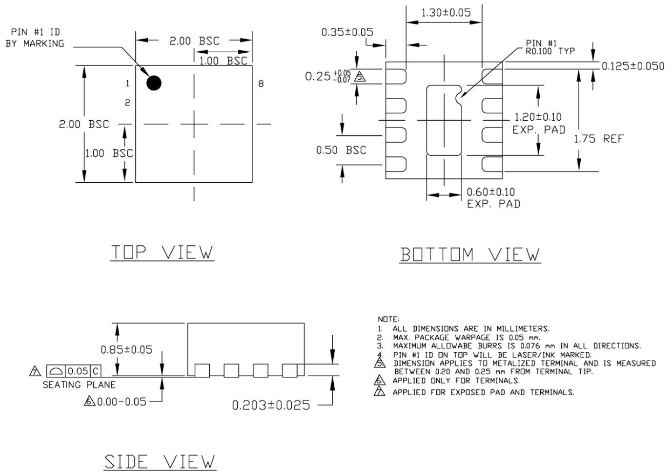
8-Pin Ultra-Small EPAD-DFN
