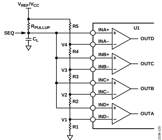
Figure 25. Programmable Sequencing Control Circuit
