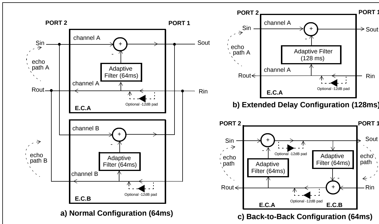
Figure 3 - Device Configuration
