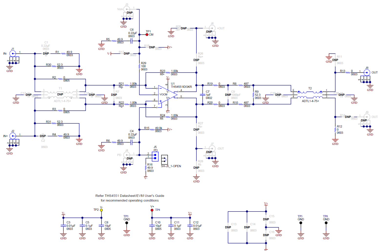
Figure 1. THS4551DGKEVM Schematic
