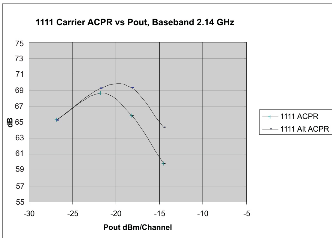
Figure 15. ACPR Versus Output Power for 4 Carriers WCDMA
