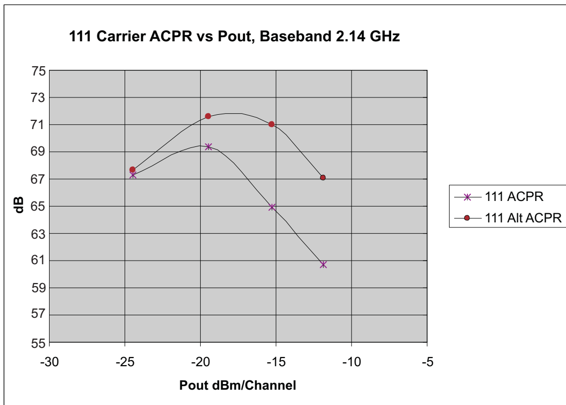
Figure 14. ACPR Versus Output Power for 3 Carriers WCDMA
