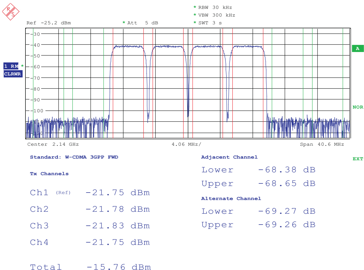
Figure 19. Optimum ACPR for 4 Carrier WCDMA, -7-dB Pad
