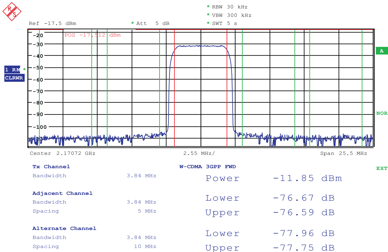
Figure 9. Single-Carrier Test Mode 1 WCDMA, Typical Performance With IF=30.72 MHz, LO=2.14 GHz
