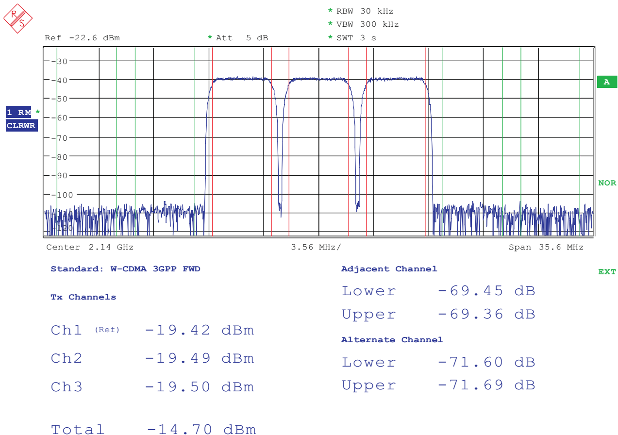
Figure 18. Optimum ACPR for 3 Carrier WCDMA, -7-dB Pad
