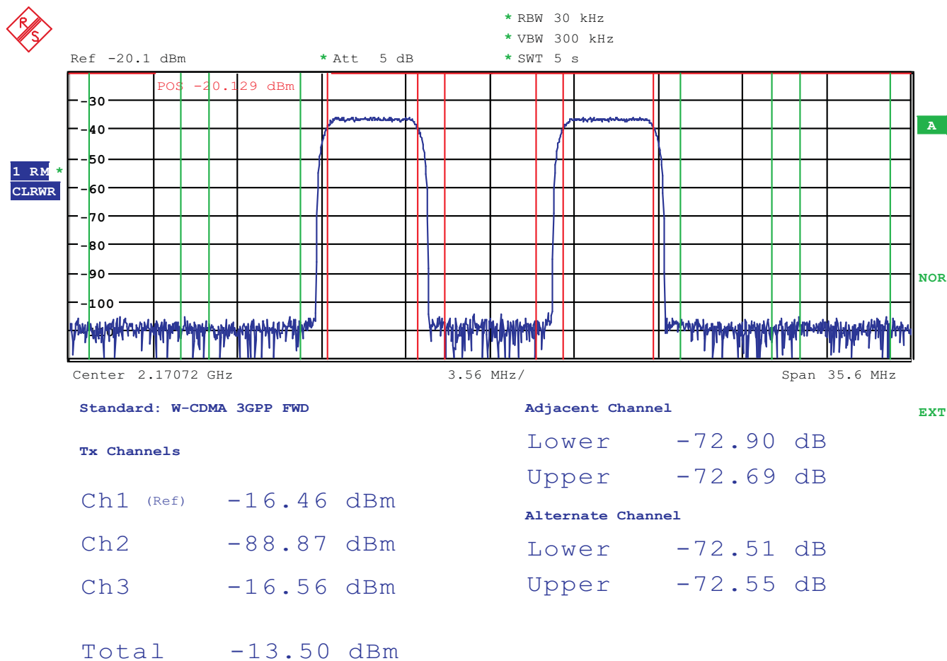
Figure 10. Missing Middle-Carrier Test Mode 1 WCDMA, Typical Performance With IF=30.72 MHz, LO=2.14 GHz
