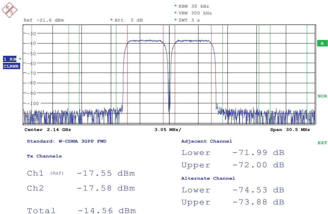
Figure 17. Optimum ACPR for 2 Carrier WCDMA, -7-dB Pad
