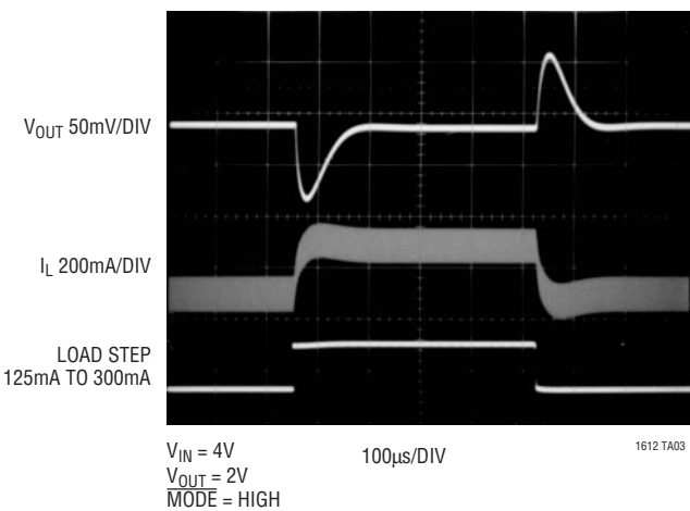
Transient Response
