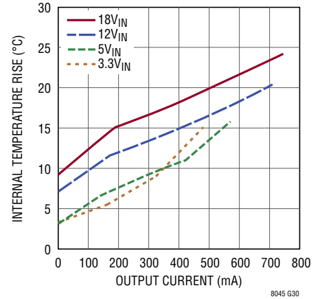
Internal Temperature Rise vs Output Current, 2.5V_{OUT} SEPIC
