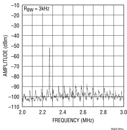
Figure 1a. Output Noise Spectrum of Conventional Buck Switching Converter (LTC3543 with Spread Spectrum Disabled) Showing Fundamental and Harmonic Frequencies
