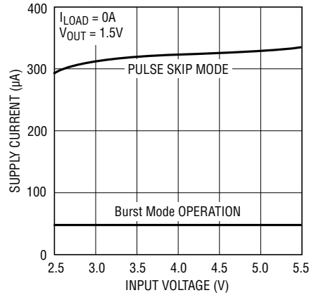
Dynamic Supply Current vs Input Voltage (V IN )
