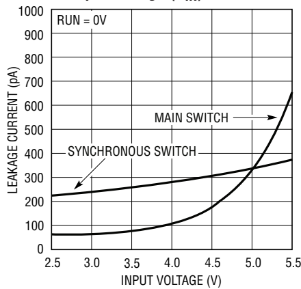
Switch Leakage (I SW ) vs Input Voltage (V IN )
