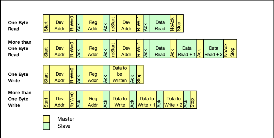
Figure 3. Operating modes
