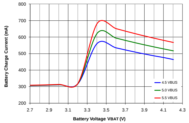
Figure 8. Battery Charge Current vs. V_{\text{BUS}} with I_{\text{BUSLIM}}=500\text{ mA}
