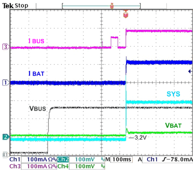
Figure 11. Charger Startup at V_{\text{BUS}} Plug-In, 100 mA I_{\text{BUSLIM}} , 3.2 V V_{\text{BAT}} , 100 \Omega SYS Load
