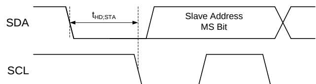
Figure 47. Start Bit
