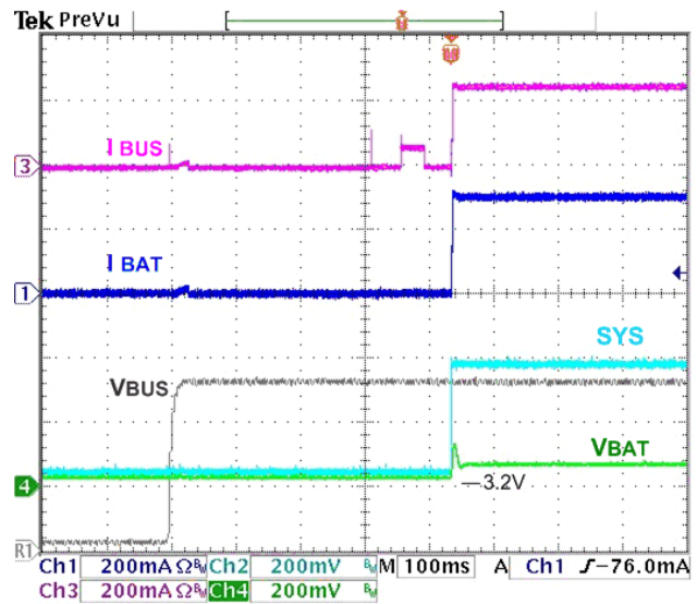
Figure 12. Charger Startup at V_{\text{BUS}} Plug-In, 500 mA I_{\text{BUSLIM}} , 3.2 V V_{\text{BAT}} , 100 \Omega SYS Load
