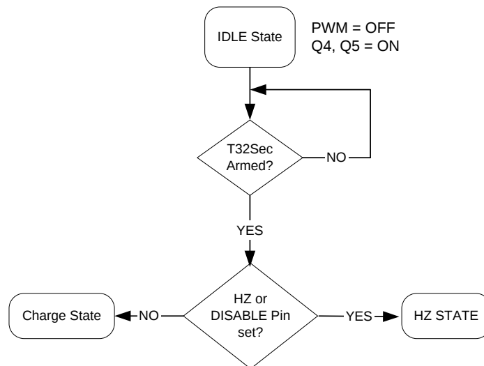
Figure 42. IDLE State
