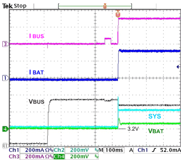
Figure 13. Charger Startup at V_{\text{BUS}} Plug-In Using 300 mA Current Limited Source, 500 mA I_{\text{BUSLIM}} , 3.2 V V_{\text{BAT}} , 50 \Omega SYS Load
