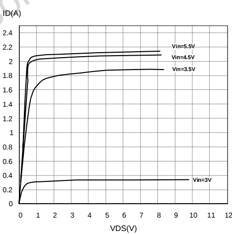
Output Characteristics
