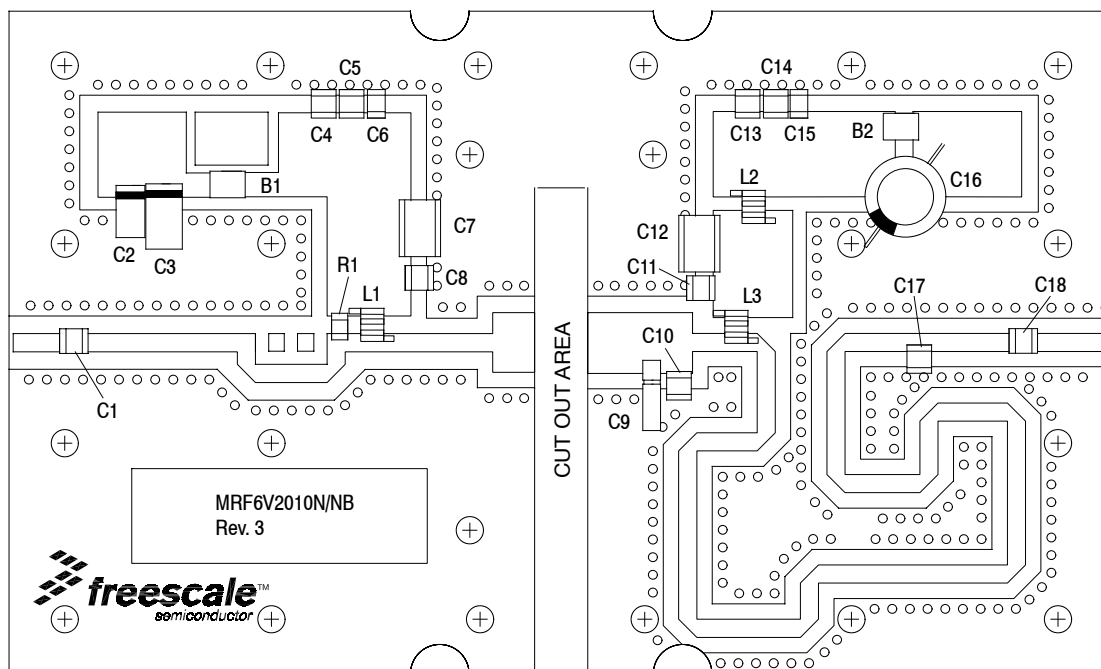
Figure 3. MRF6V2010N(NB) Test Circuit Component Layout
