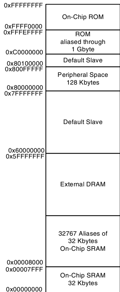
Figure 1-3. Physical Memory Map
