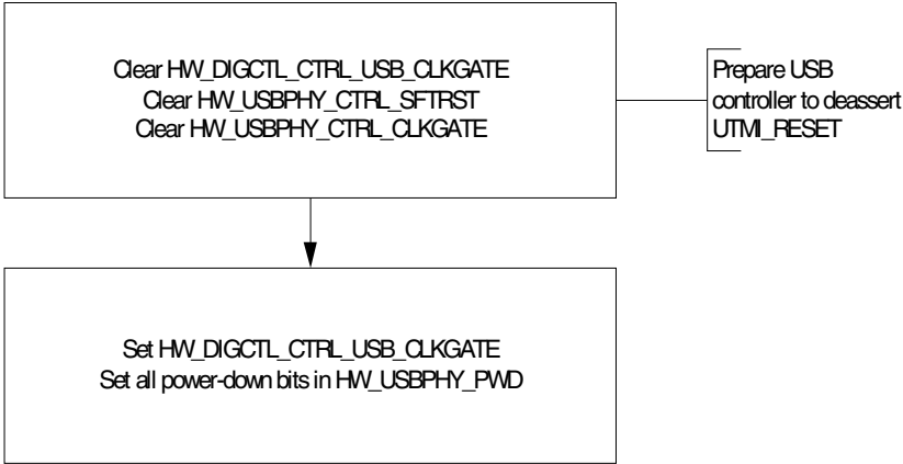
Figure 8-5. UTMI Powerdown
