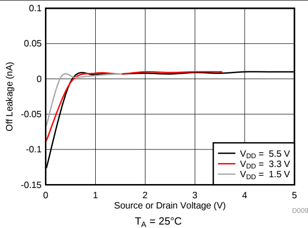
Figure 9. Off-Leakage vs Source or Drain Voltage
