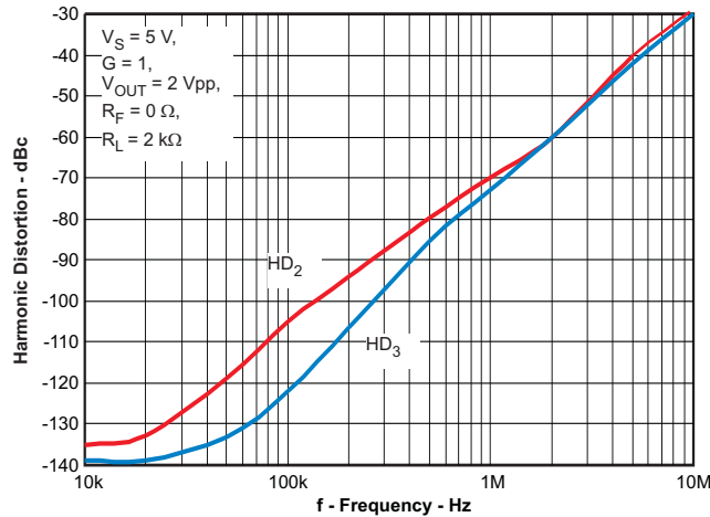
Figure 33. Harmonic Distortion vs Frequency
