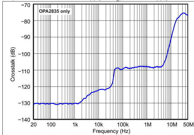
Figure 19. Crosstalk vs Frequency
