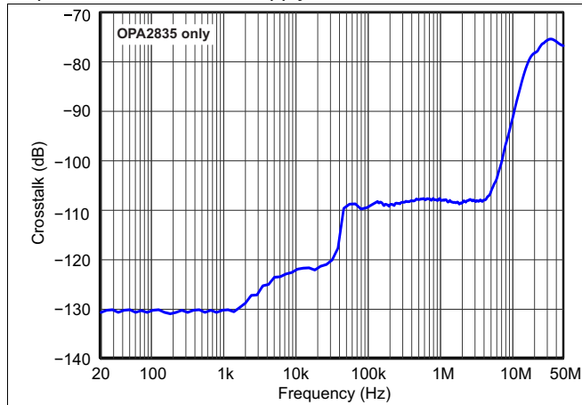
Figure 45. Crosstalk vs Frequency
