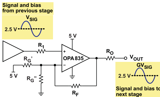
Figure 61. Noninverting Single Supply With Resistors
