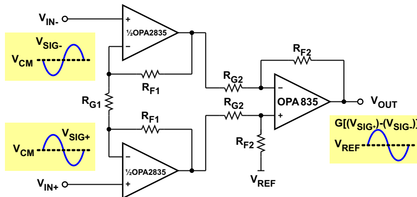
Figure 64. Instrumentation Amplifier
