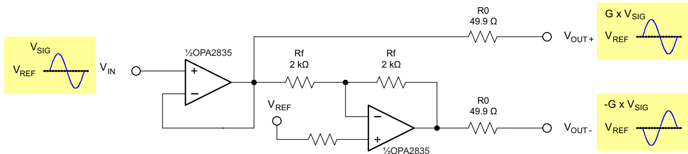
Figure 66. Cat5 Line Driver With Gain = 2 V/V (6 dB)
