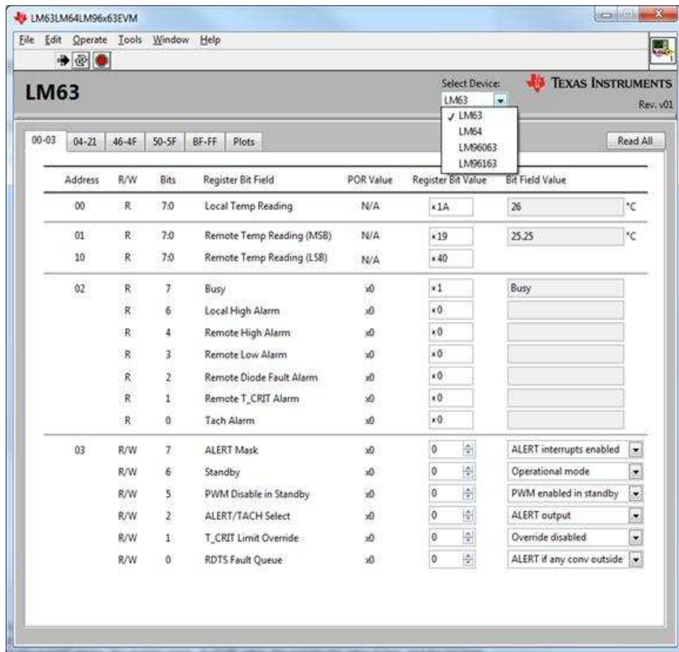
Figure 28. Part Select
