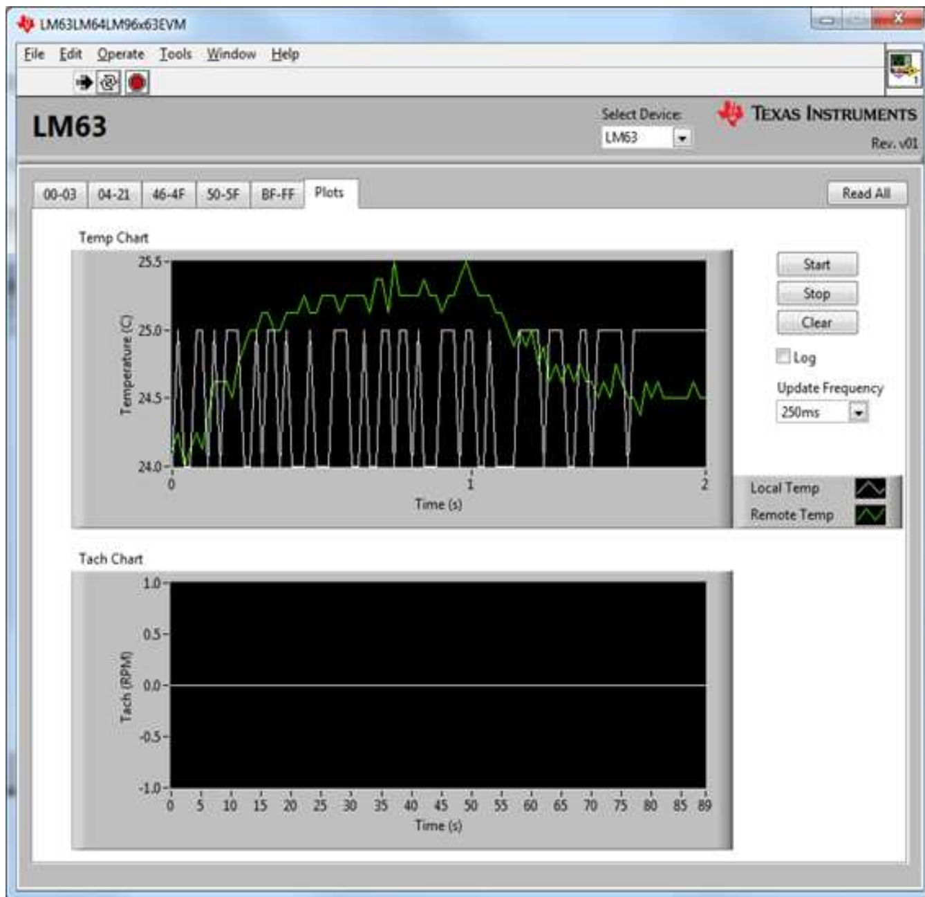
Figure 30. Plots Tab
