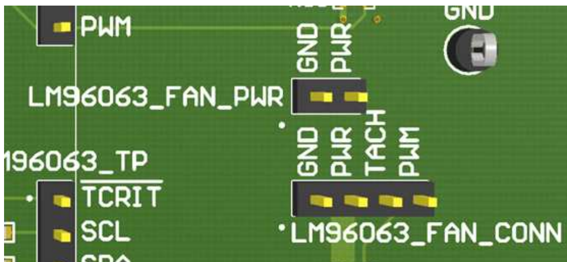
Figure 16. LM96063 Fan Connector
