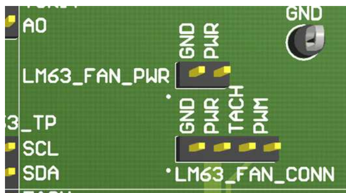
Figure 14. LM63 Fan Connector
