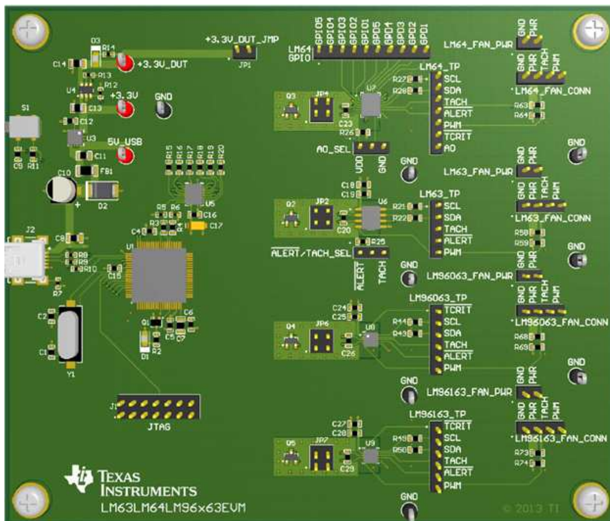
Figure 1. LM63LM64LM96x63EVM Board
