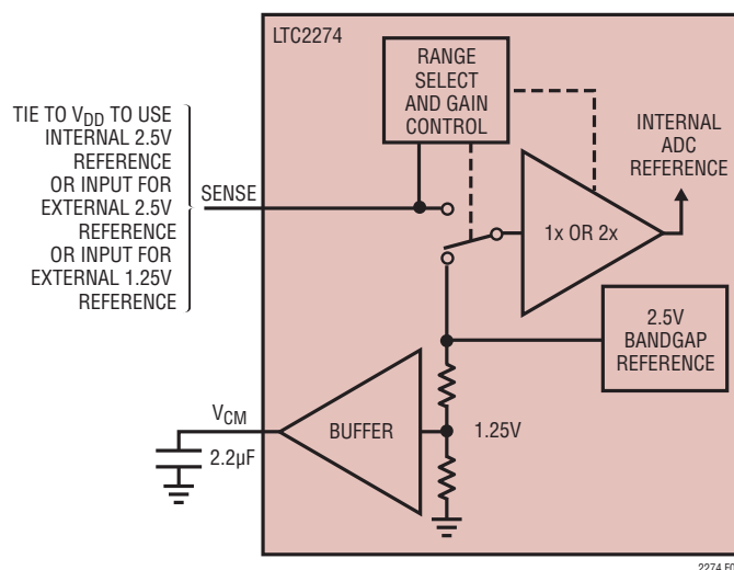
Figure 6. Reference Circuit
