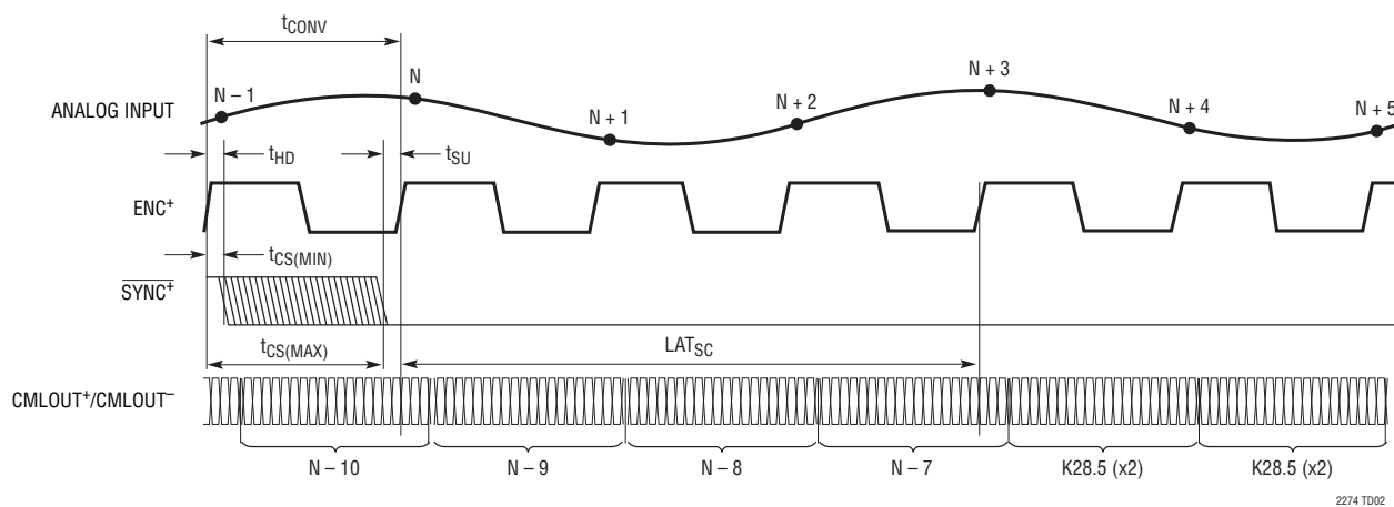
SYNC^+ Falling Edge to Comma (K28.5) Timing
