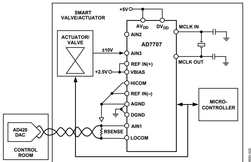
Figure 26. Smart Valve/Actuator Control Using the AD7707
