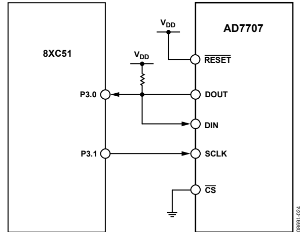
Figure 24. AD7707-to-8XC51 Interface
