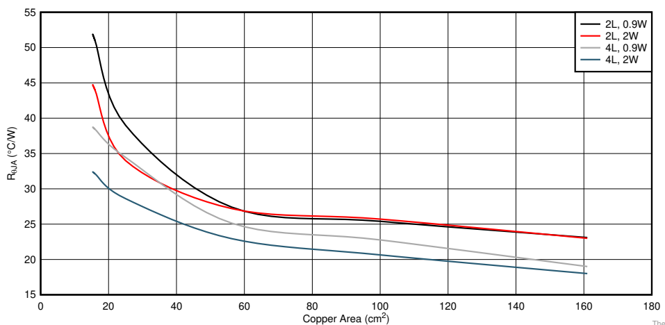
Figure 24. Typical R_{\theta JA} vs Copper Area for the WSON Package
