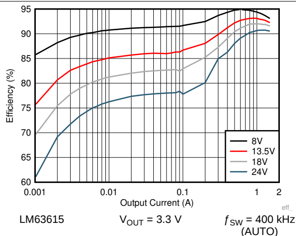
Figure 33. Efficiency
