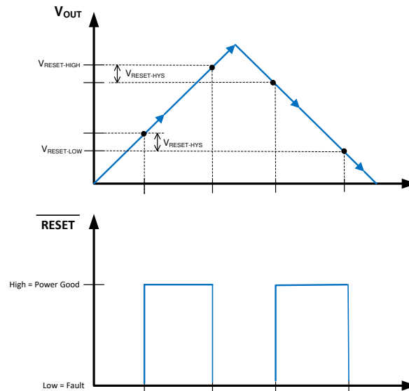
Figure 8. Static \overline{\text{RESET}} Operation
