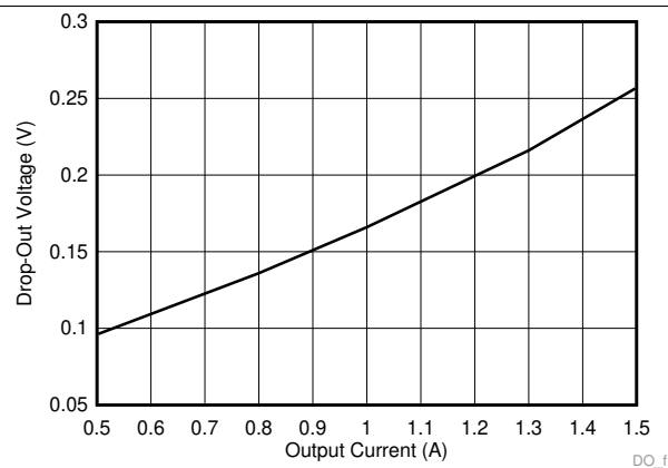
Figure 53. Dropout Voltage versus Output Current for -1% Drop
