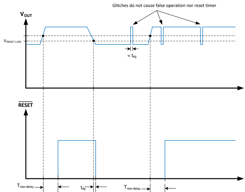
Figure 9. \overline{\text{RESET}} Timing Behavior
