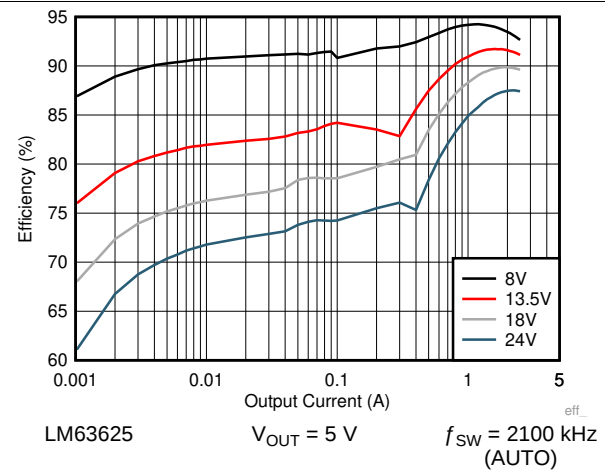
Figure 28. Efficiency
