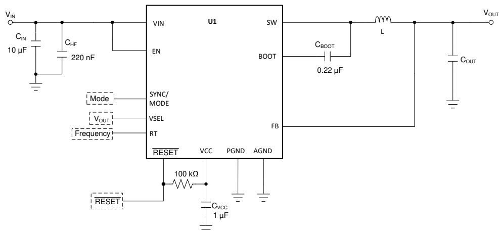
Figure 63. Circuit for Typical Application Curves
