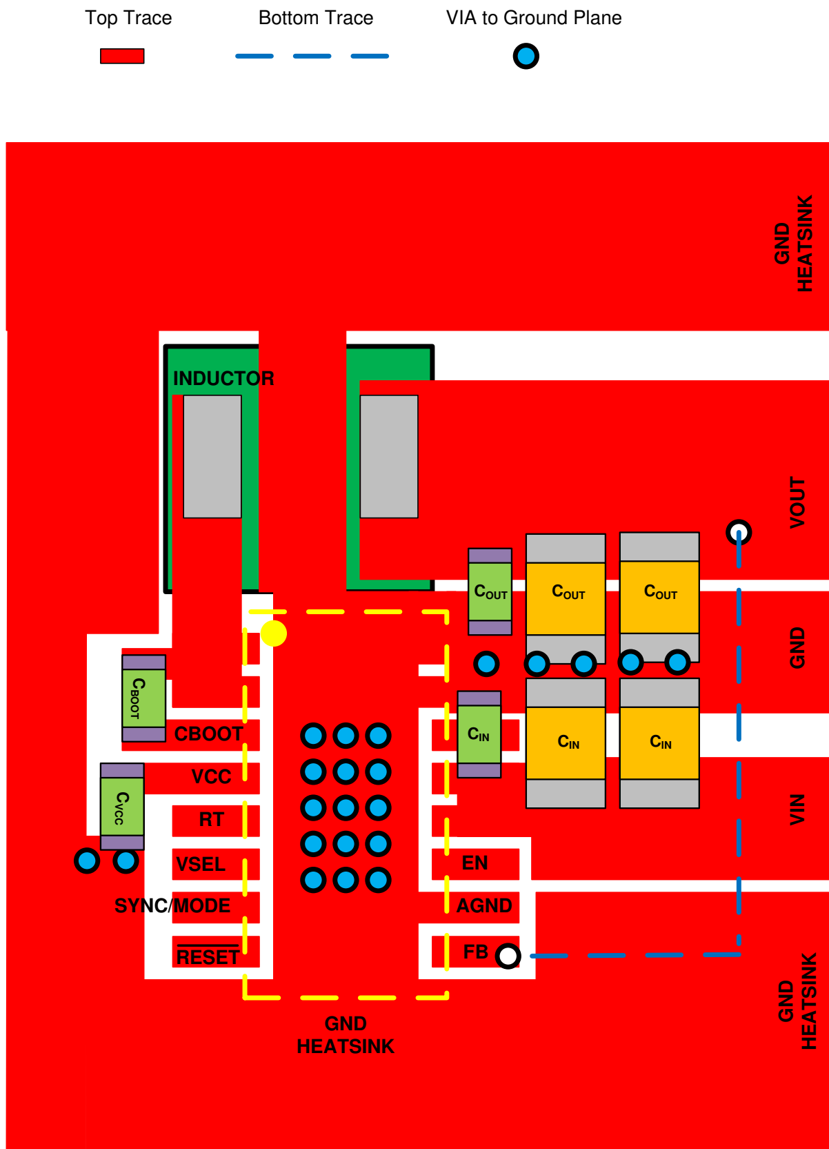
Figure 68. Example Layout for HTSSOP Package
