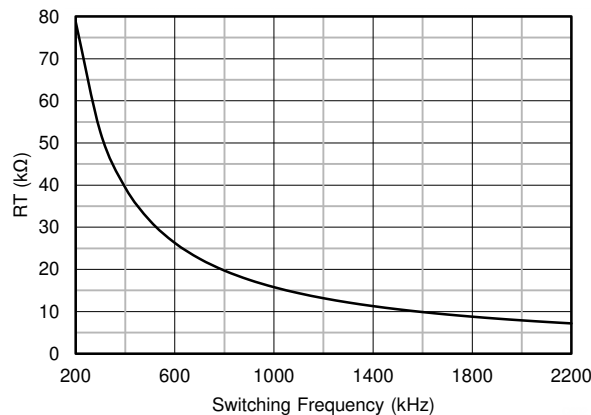
Figure 5. Switching Frequency versus R_T
