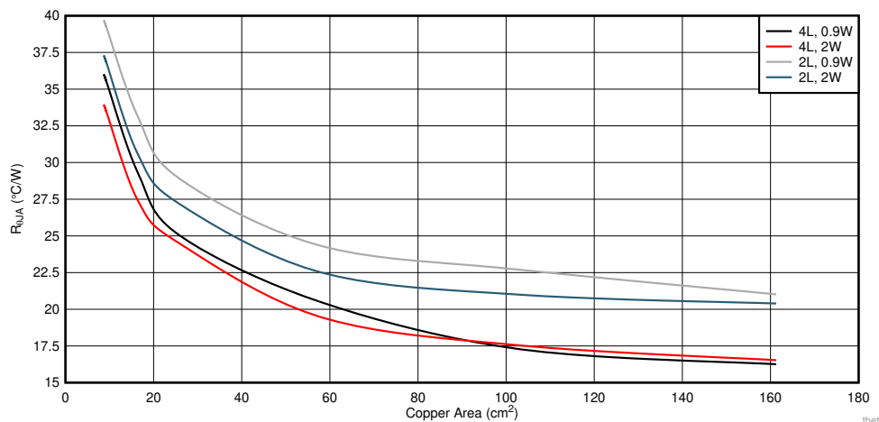
Figure 23. Typical R_{\theta JA} versus Copper Area for the HTSSOP Package
