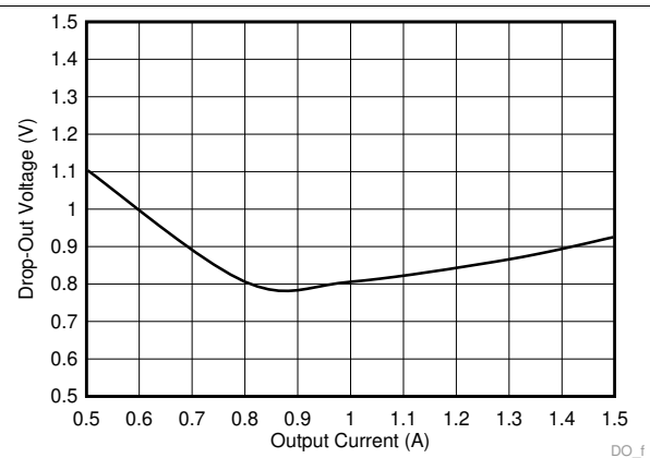
Figure 54. Dropout Voltage versus Output Current to 1.85 MHz
