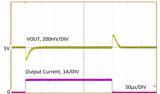
Figure 46. Load Transient
