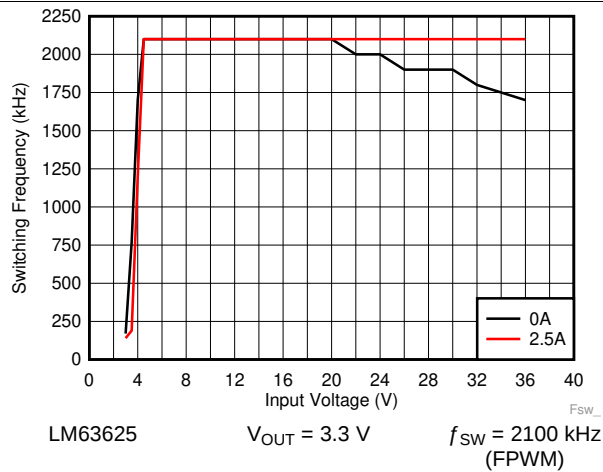
Figure 41. Switching Frequency versus Input Voltage
