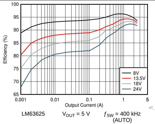
Figure 27. Efficiency
