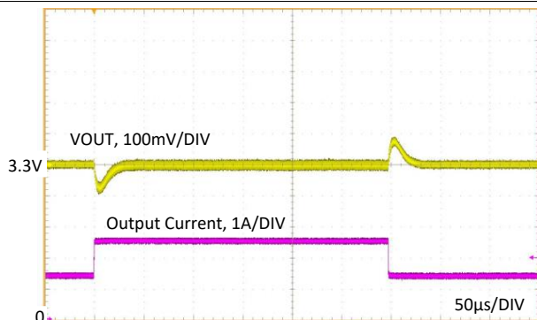
Figure 47. Load Transient
