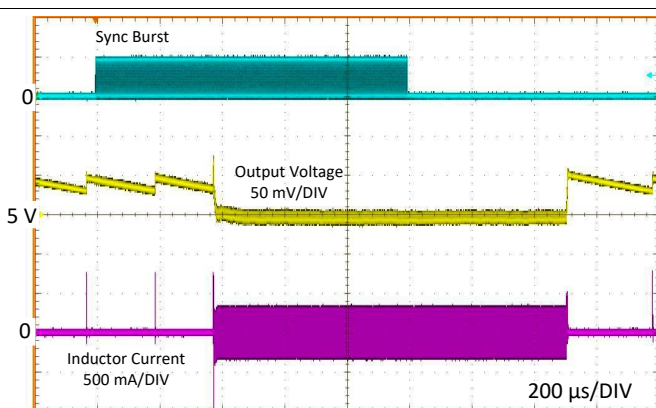
Figure 15. Typical Transition from Sync Mode to FPWM Mode V_{IN} = 12\text{ V} , V_{OUT} = 5\text{ V} , I_{OUT} = 1\text{ mA}
