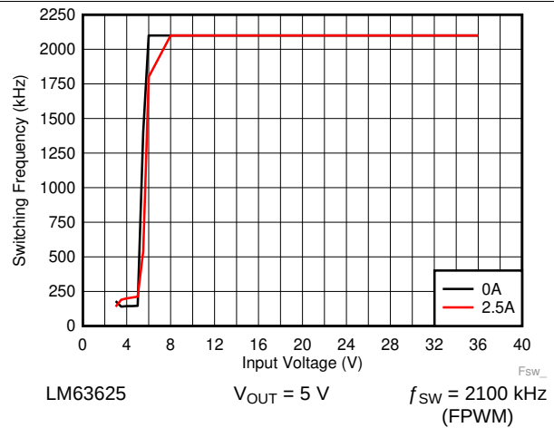
Figure 42. Switching Frequency versus Input Voltage
