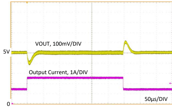
LM63625 V_{OUT} = 5\text{ V} f_{SW} = 2100\text{ kHz} 1.5 A to 2.5 A, 2 \mu\text{s} AUTO
