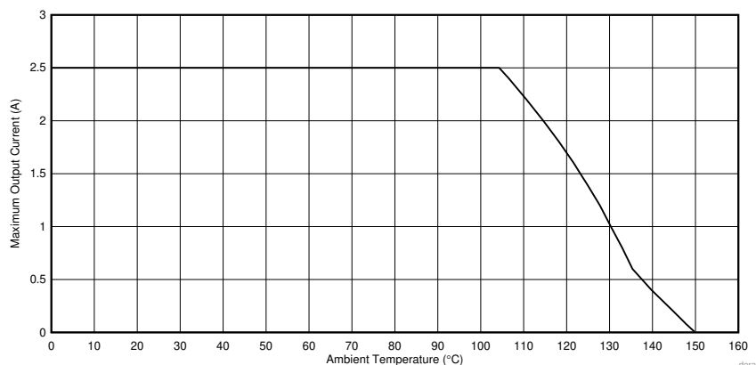
Figure 25. Maximum Output Current versus Ambient Temperature V_{IN} = 12\text{ V} , V_{OUT} = 5\text{ V} , f_{SW} = 2.1\text{ MHz} , R_{\theta JA} = 30^{\circ}\text{C/W}
