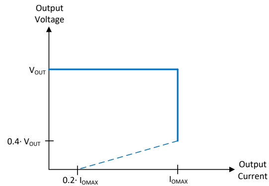
Figure 19. Output Voltage versus Output Current in Current Limit
