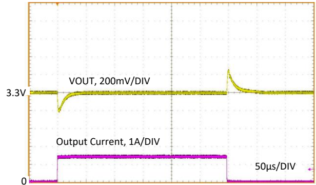
LM63615 V_{OUT} = 3.3\text{ V} f_{SW} = 2100\text{ kHz} 0 A to 1.5 A, 2 \mu\text{s} FPWM
