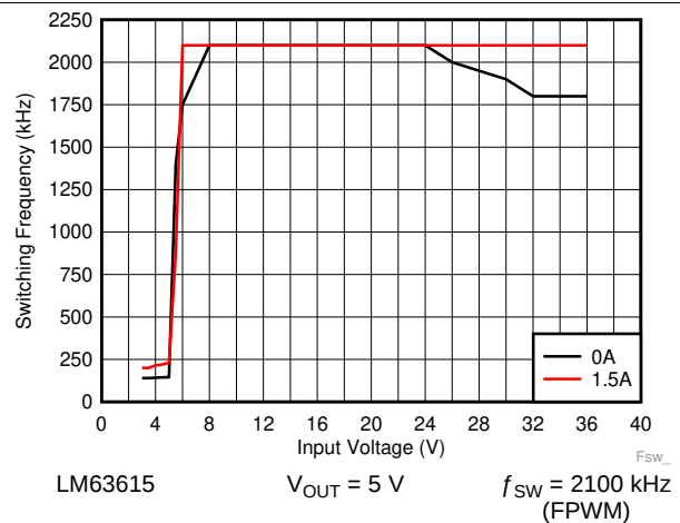
Figure 44. Switching Frequency versus Input Voltage
