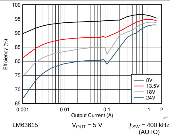
Figure 29. Efficiency
