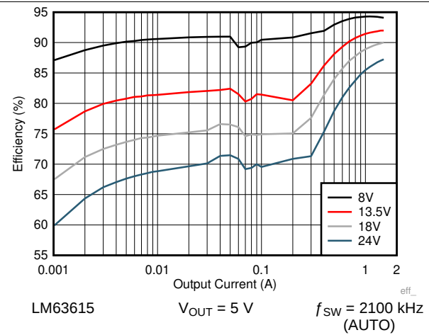
Figure 30. Efficiency
