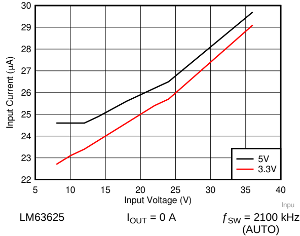
Figure 57. Input Supply Current versus Input Voltage
