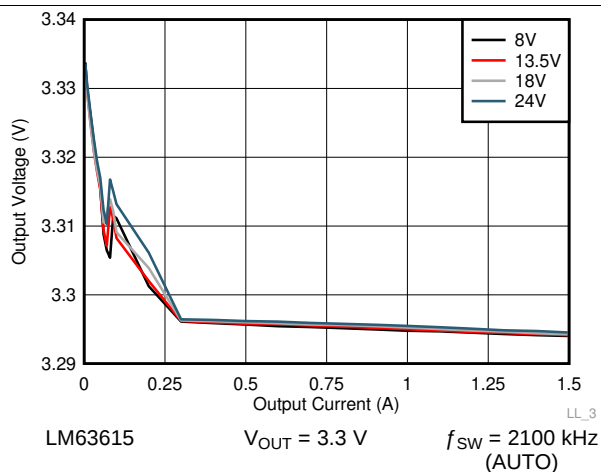
Figure 38. Line and Load Regulation
