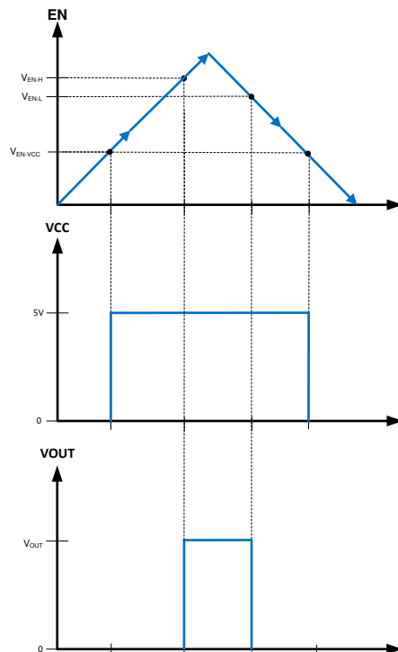
Figure 6. Precision Enable Behavior
