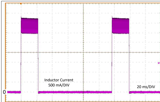
Figure 17. Inductor Current Burst in Short-Circuit Mode; LM63625
