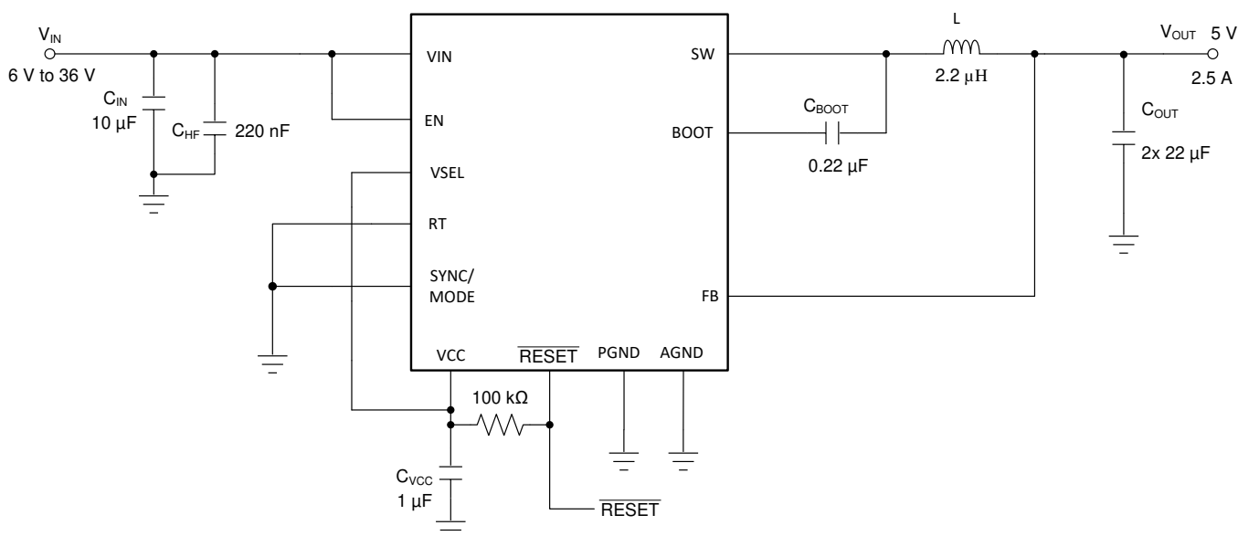
Figure 20. Example Application Circuit V_{IN} = 12\text{ V} , V_{OUT} = 5\text{ V} , I_{OUT} = 2.5\text{ A} , f_{SW} = 2.1\text{ MHz}
