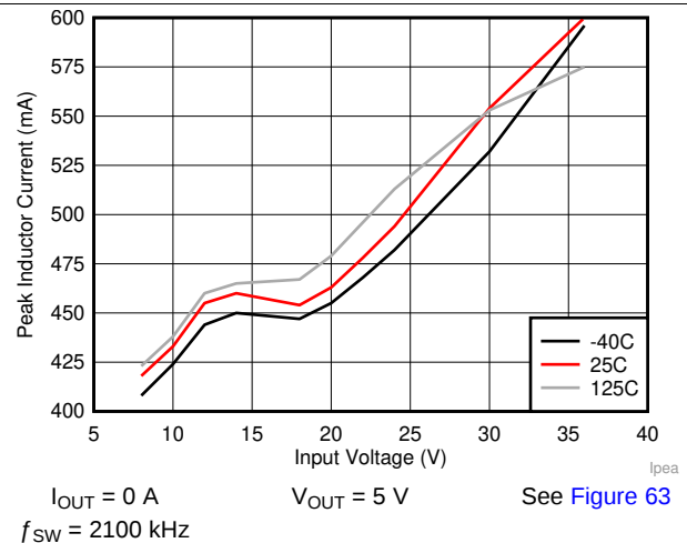
Figure 4. I_{PEAK-MIN} for LM63615
