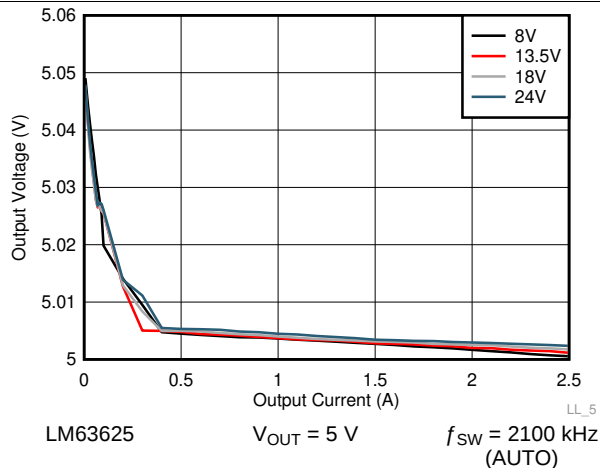
Figure 35. Line and Load Regulation
