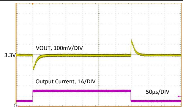
Figure 48. Load Transient
