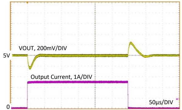
Figure 45. Load Transient
