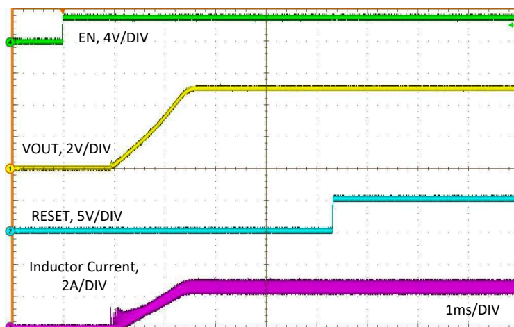
Figure 6. Precision Enable Behavior
