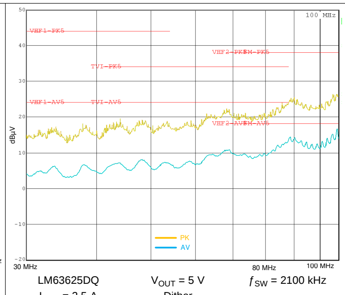
Figure 65. Typical Conducted EMI 30 MHz to 108 MHz
