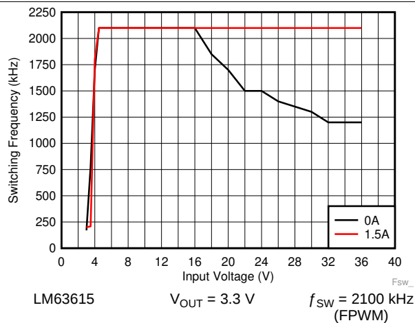
Figure 43. Switching Frequency versus Input Voltage
