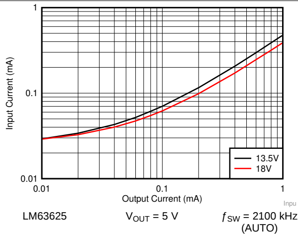
Figure 59. Input Supply Current versus Output Current
