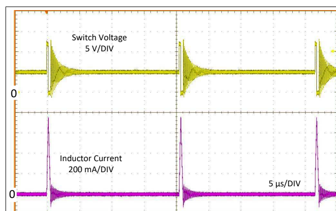
Figure 10. Typical PFM Switching Waveforms V_{IN} = 12\text{ V} , V_{OUT} = 5\text{ V} , I_{OUT} = 10\text{ mA}
