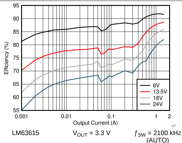
Figure 34. Efficiency
