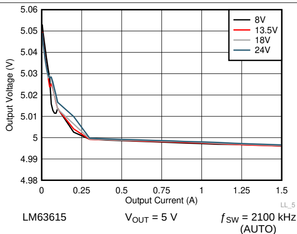
Figure 37. Line and Load Regulation
