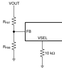
Figure 21. Feedback Divider for Adjustable Output Voltage Setting
