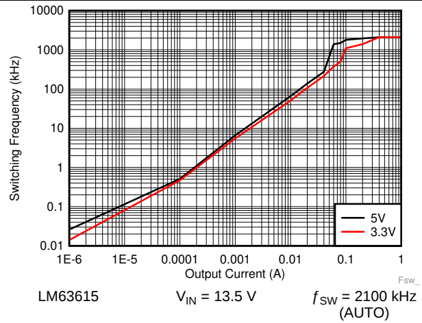
Figure 40. Switching Frequency versus Output Current
