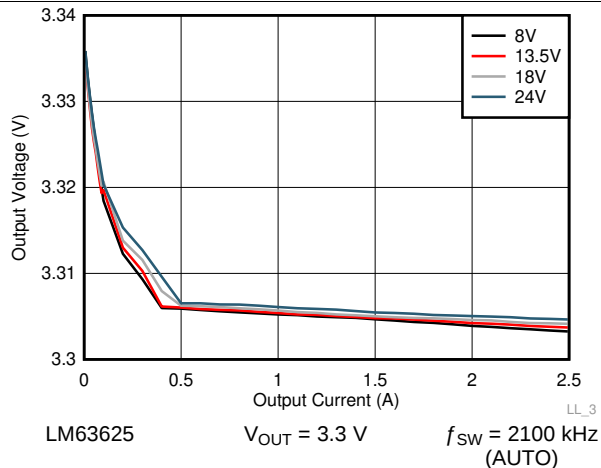
Figure 36. Line and Load Regulation
