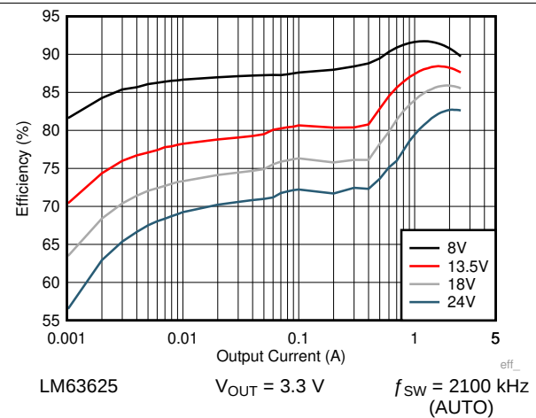
Figure 32. Efficiency
