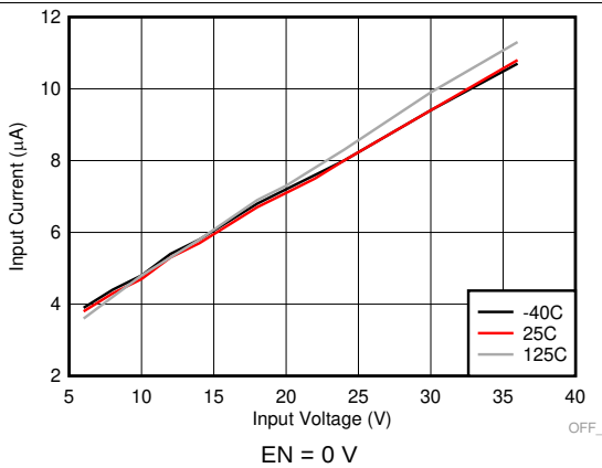
Figure 1. Input Supply Current in Shutdown Mode
