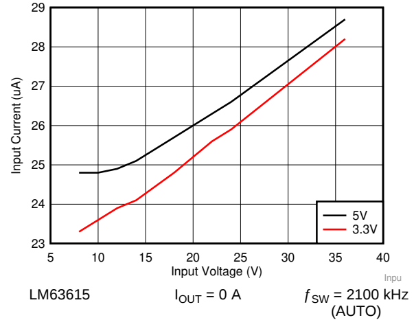
Figure 58. Input Supply Current versus Input Voltage
