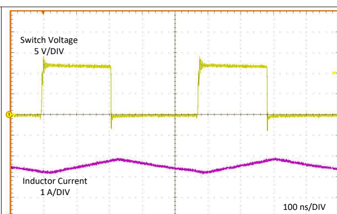
Figure 11. Typical PWM Switching Waveforms Without Spread Spectrum V_{IN} = 12\text{ V} , V_{OUT} = 5\text{ V} , I_{OUT} = 2.5\text{ A} , f_{SW} = 2100\text{ kHz}
