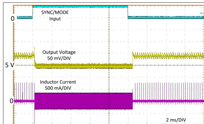
Figure 14. Typical Transition from FPWM to AUTO Mode V_{IN} = 12\text{ V} , V_{OUT} = 5\text{ V} , I_{OUT} = 1\text{ mA}
