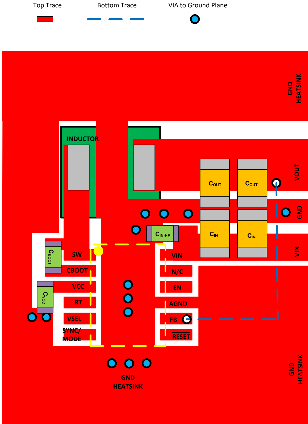
Figure 69. Example Layout for WSON Package
