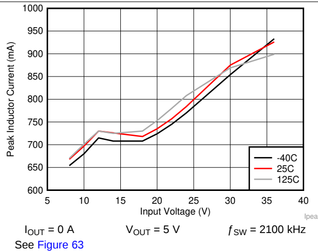
Figure 3. I_{PEAK-MIN} for LM63625
