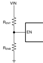
Figure 22. Setup for External UVLO Application
