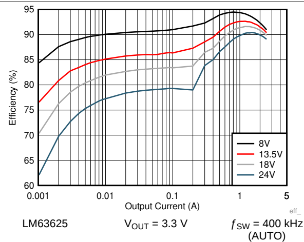
Figure 31. Efficiency
