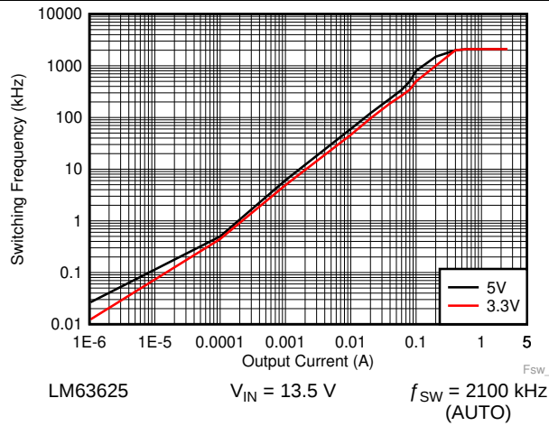
Figure 39. Switching Frequency versus Output Current
