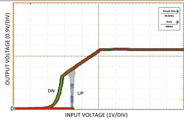
Figure 2. UVLO Thresholds
