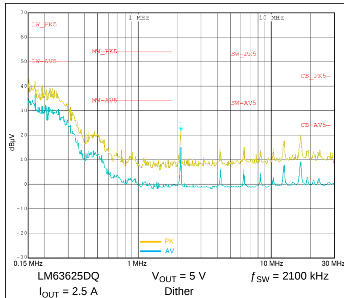
Figure 64. Typical Conducted EMI 0.15 MHz to 30 MHz
