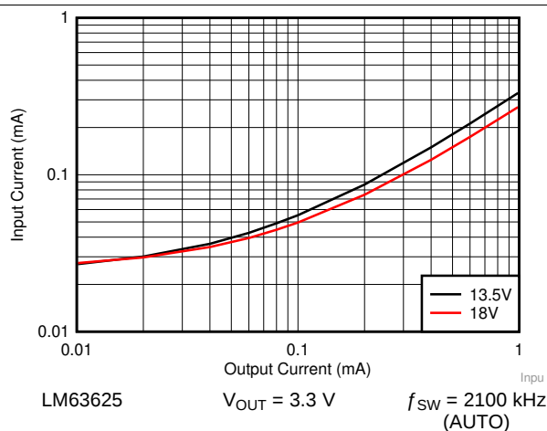
Figure 61. Input Supply Current versus Output Current
