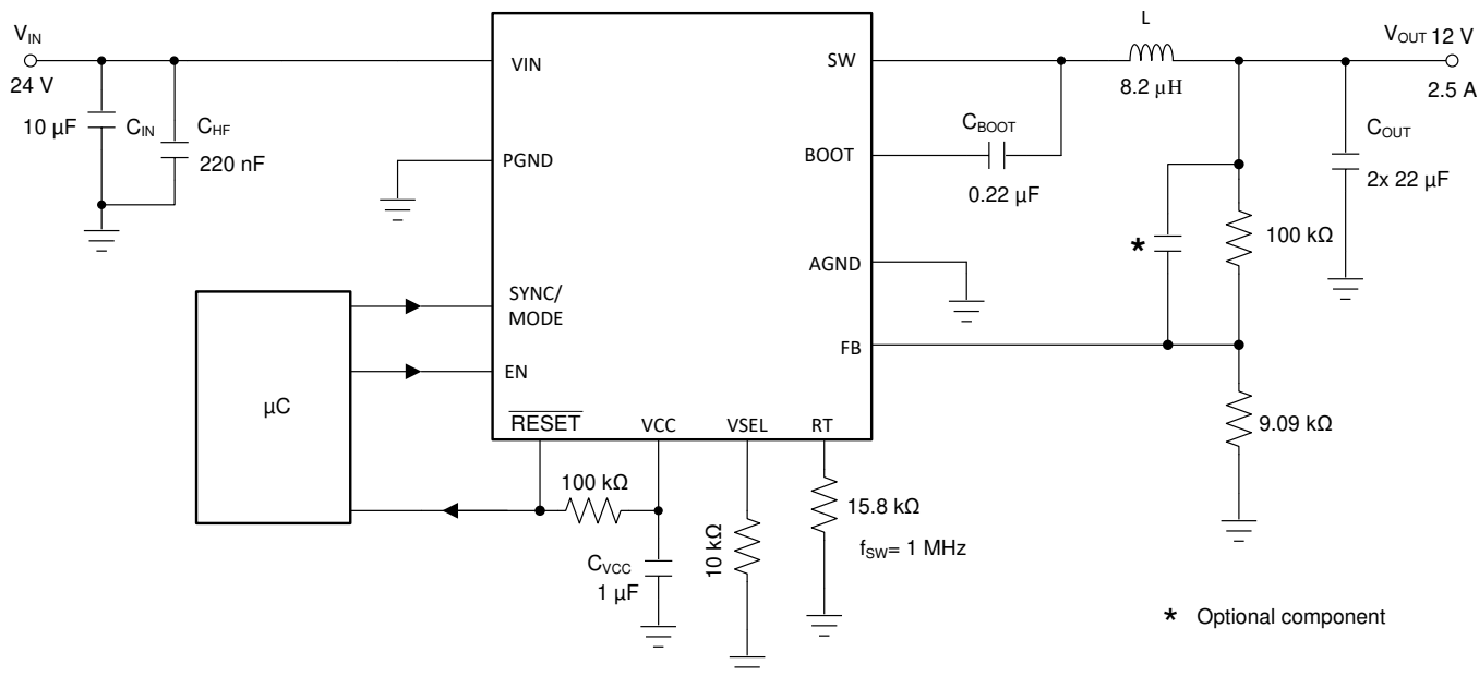
Figure 26. Full-Featured Design Example V_{IN} = 24\text{ V} , V_{OUT} = 12\text{ V} , I_{OUT} = 2.5\text{ A} , f_{SW} = 1\text{ MHz}
