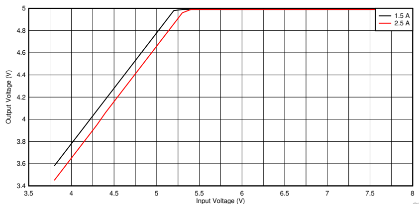
Figure 16. Overall Dropout Characteristic V_{OUT} = 5\text{ V}
