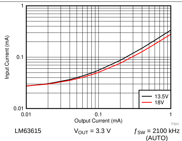
Figure 62. Input Supply Current versus Output Current
