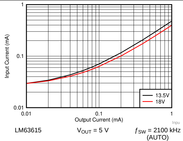
Figure 60. Input Supply Current versus Output Current
