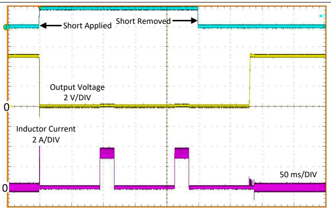
Figure 18. Short-Circuit Transient and Recovery; LM63625
