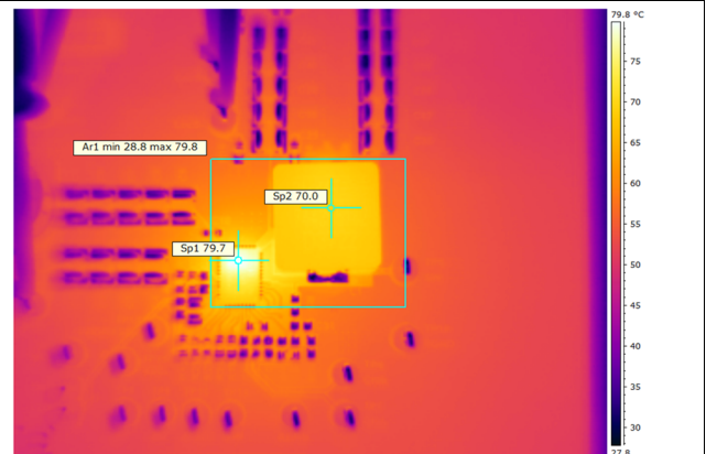
Figure 10. Thermal Image
