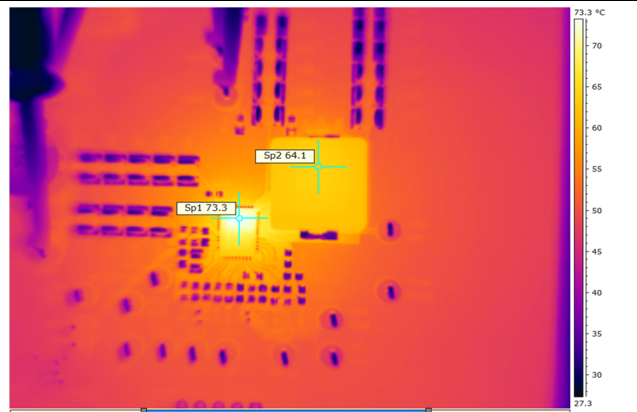
Figure 9. Thermal Image
