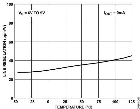
Figure 7. Line Regulation vs. Temperature
