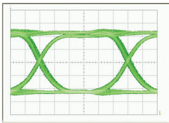
Eye Diagram
