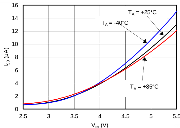
Figure 39. Standby Current vs. V_{IN} EN = 1.8\text{V}
