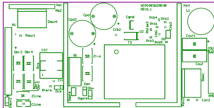
Figure 5. Silkscreen Front
