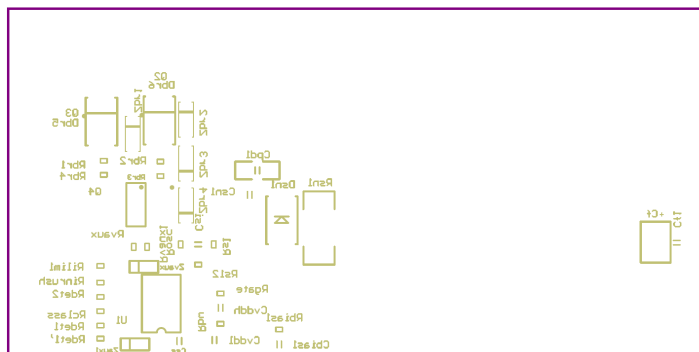
Figure 6. Silkscreen Back
