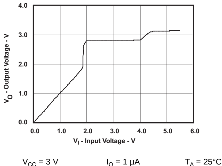
Figure 10. Data Output Voltage vs Data Input Voltage
