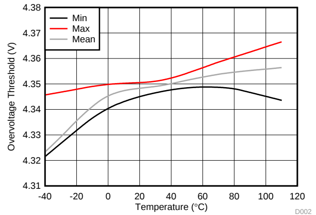
Figure 2. bq294602 Overvoltage Threshold (OVT) vs Temperature
