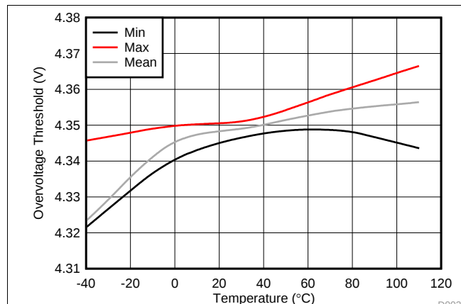
Figure 9. OVT vs Temperature
