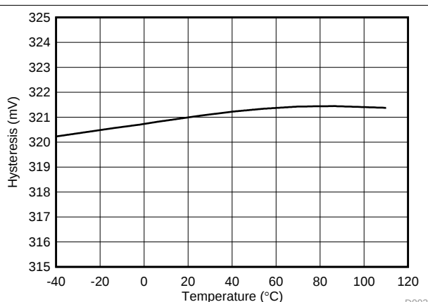
Figure 10. V_{HYS} vs Temperature
