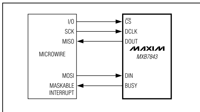
Figure 11. MICROWIRE Interface
