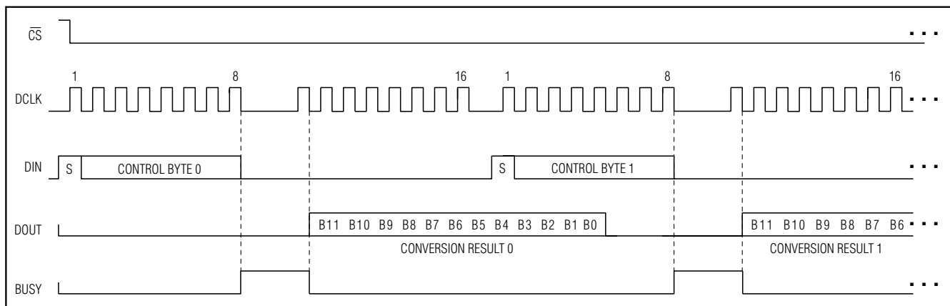
Figure 9. 16-Clock/Conversion Timing
