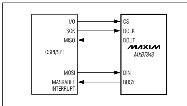
Figure 12. QSPI/SPI Interface
