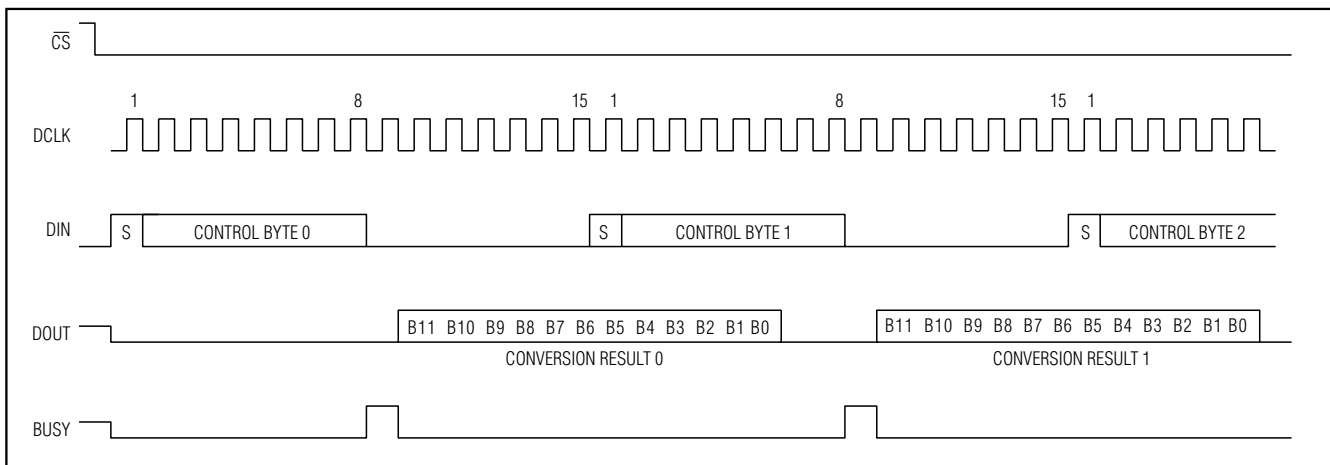
Figure 8. 15-Clock/Conversion Timing
