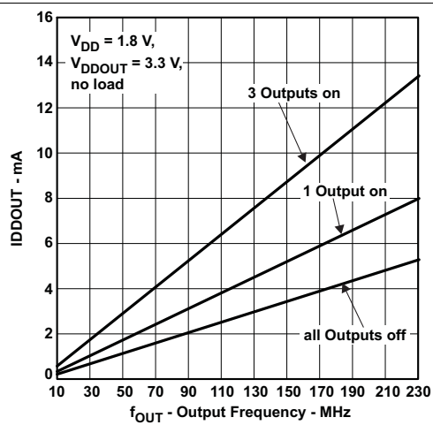
Figure 2. CDCE813-Q1 Output Current vs Output Frequency
