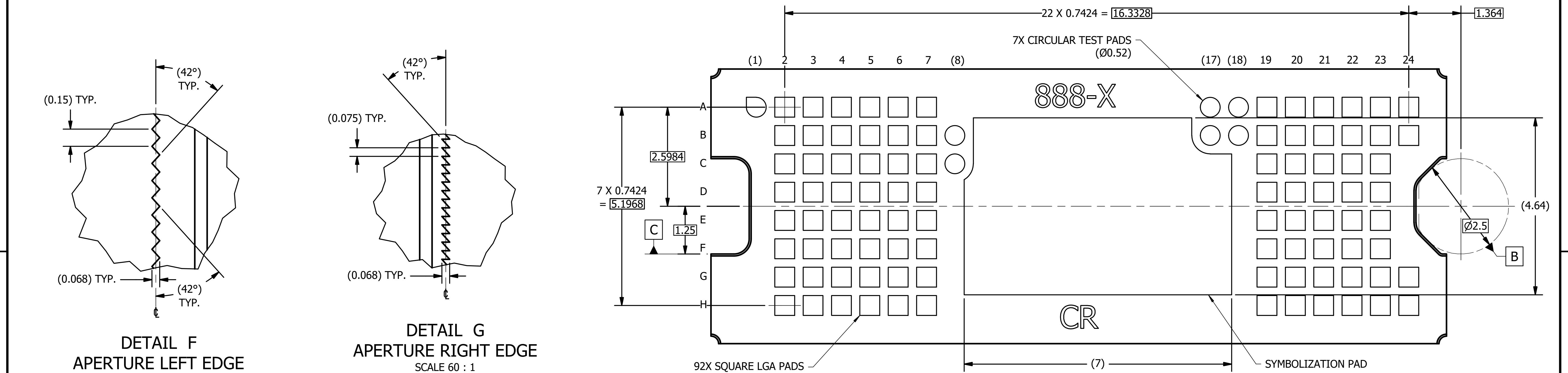
VIEW H-H BACK SIDE METALLIZATION (FROM SHEET 1)
