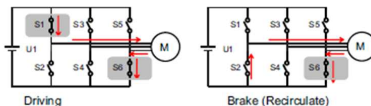
Figure 13. IPD Release Mode 0 – Brake Mode
