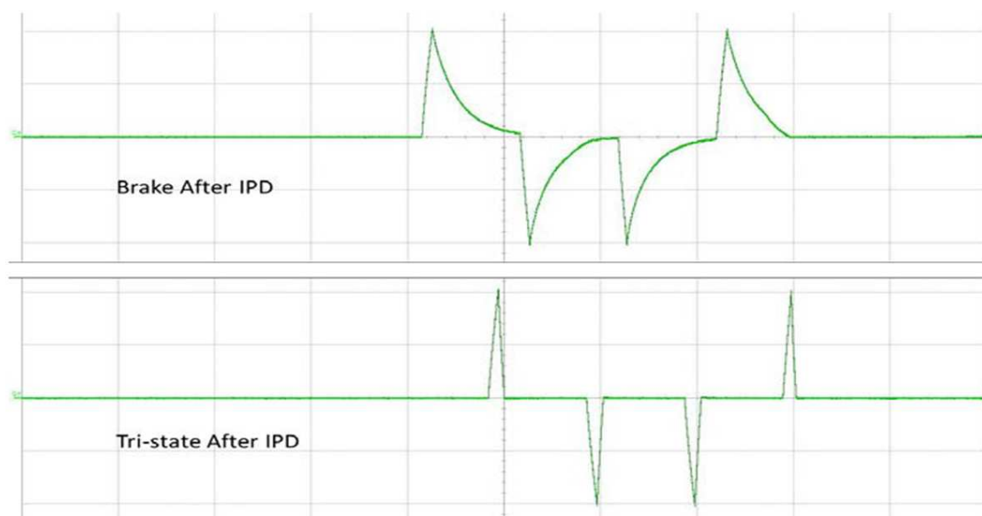
Figure 16. Brake Versus Tri-State After IPD
