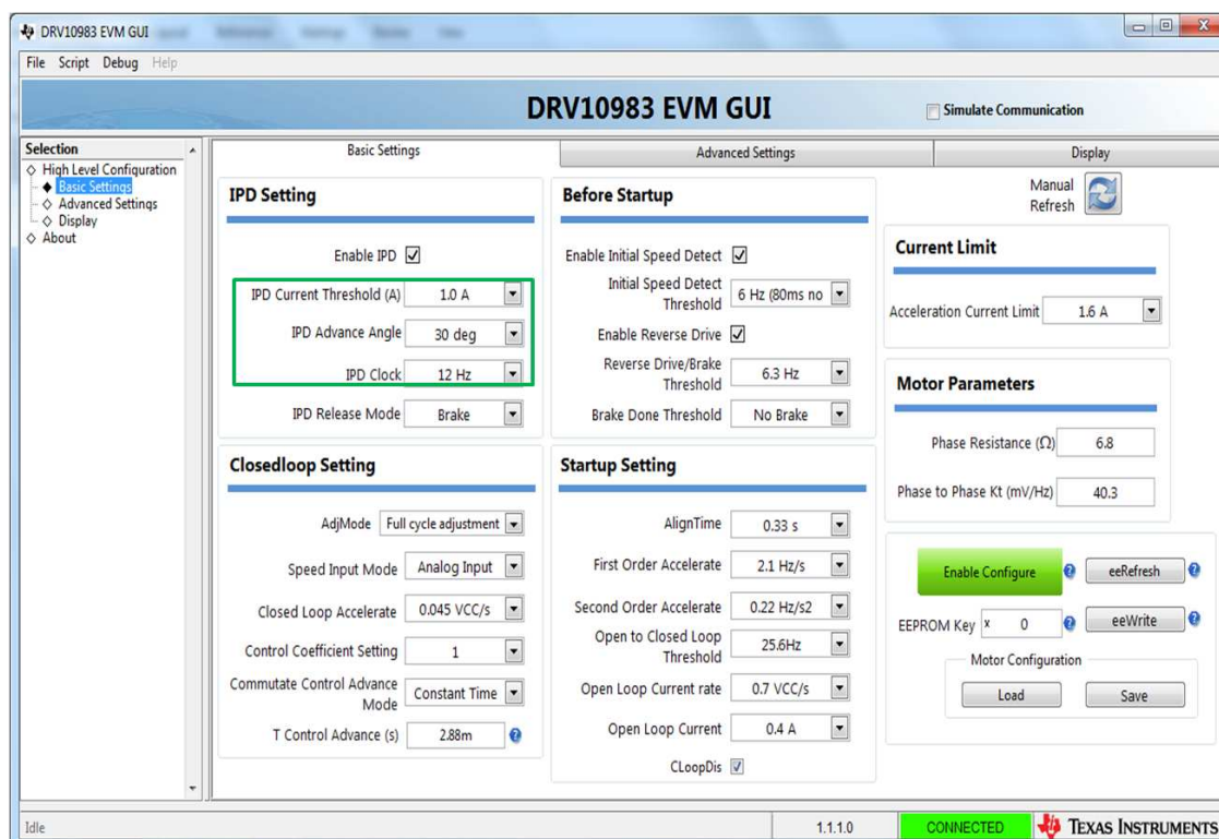
Figure 9. DRV10983x/75 EVM GUI Screenshot
