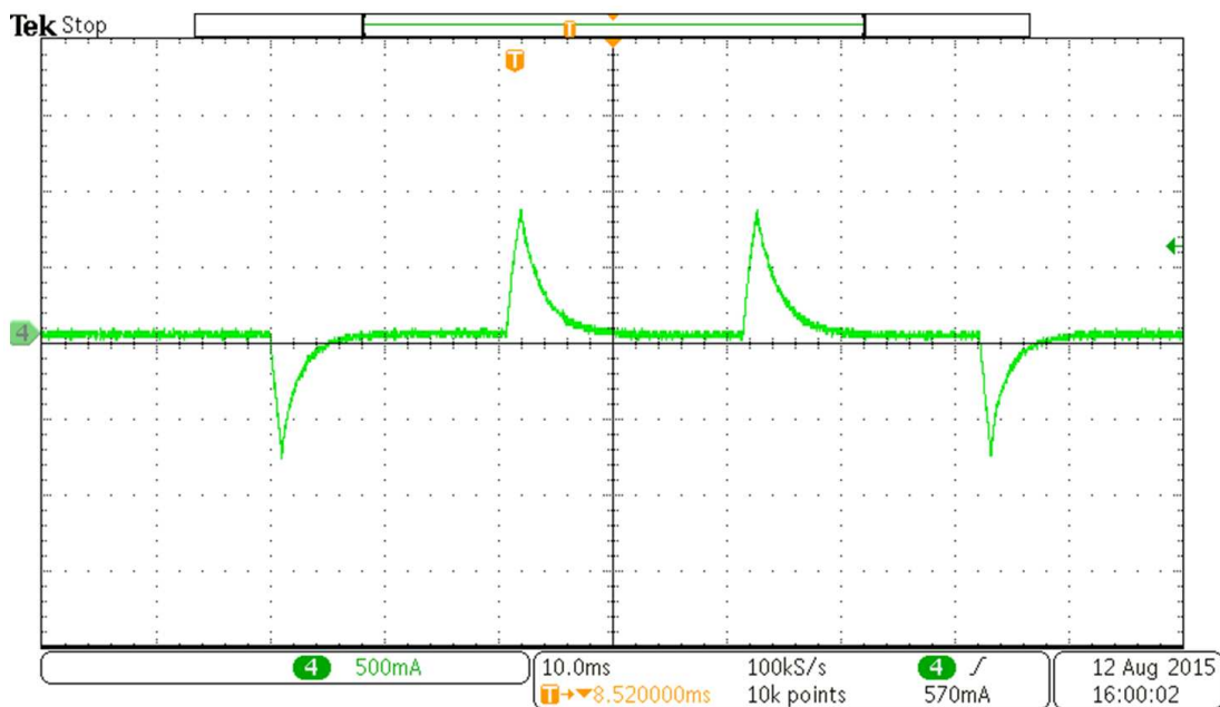
Figure 39. Motor Phase Current With 47-Hz IPD Clock
