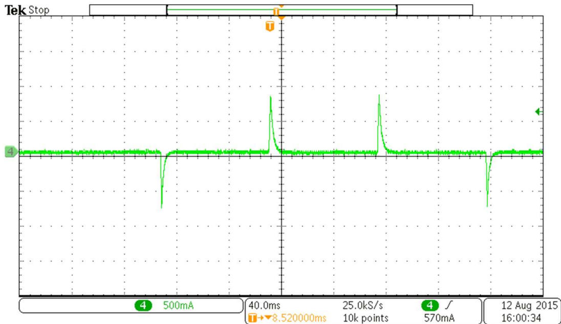
Figure 35. Motor Phase Current With 12-Hz IPD Clock
