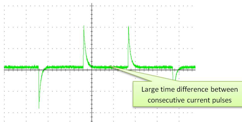
Figure 19. Current Waveform During IPD Process With Low 'IPD Clock' Frequency
