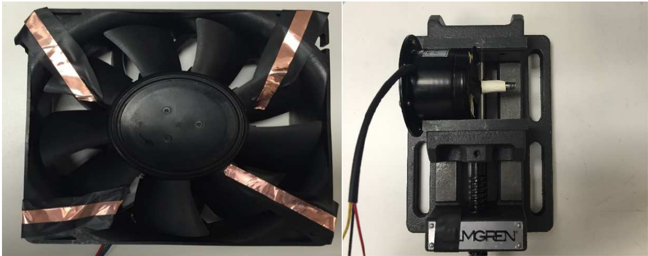
Figure 6. Rotor of Motor Locked to its Position Using Clamp and Insulation Tape
