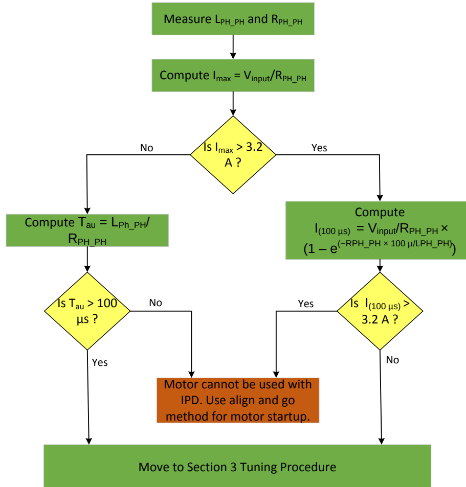
Figure 4. Flowchart for Preliminary Check of Motor for IPD Algorithm Suitability
