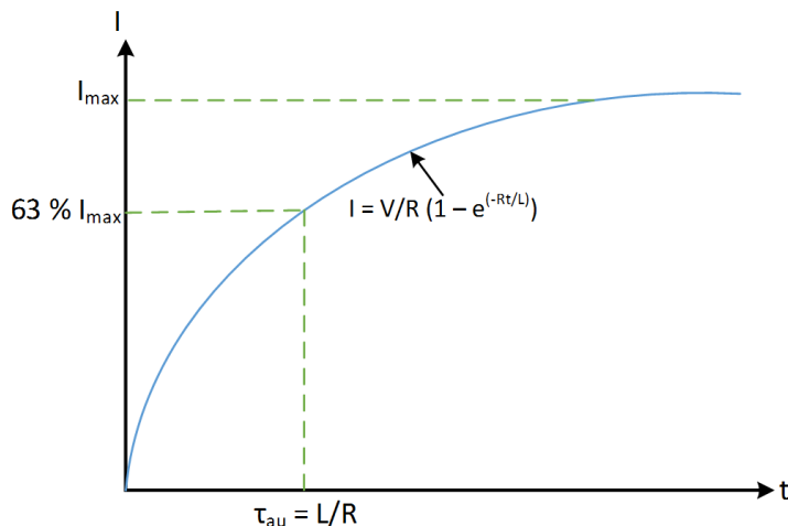
Figure 24. Step Response of Series LR Circuit
