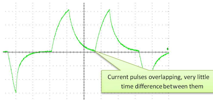
Figure 20. Current Waveform During IPD Process With High 'IPD Clock' Frequency
