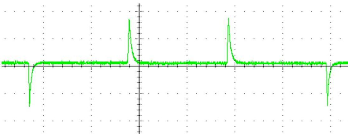
Figure 32. Motor Phase Current During Brake Mode
