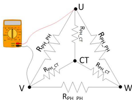
Figure 2. Motor Resistance Measurements
