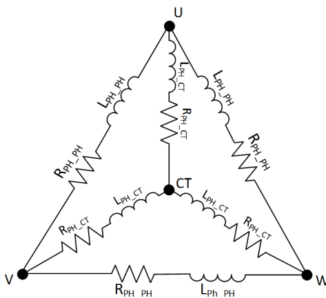
Figure 23. Motor Windings With Series Phase Resistance and Phase Inductance
