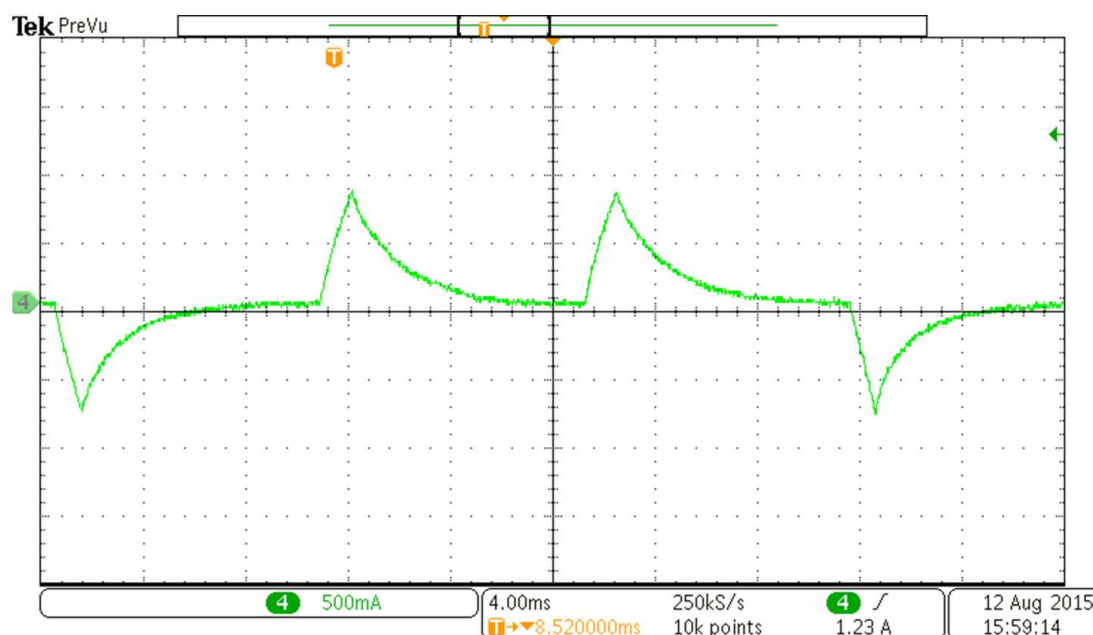
Figure 41. Motor Phase Current With 95-Hz IPD Clock
