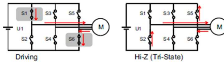
Figure 14. IPD Release Mode 1 – Tri-State Mode
