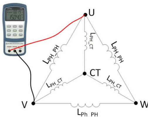
Figure 3. Motor Inductance Measurements
