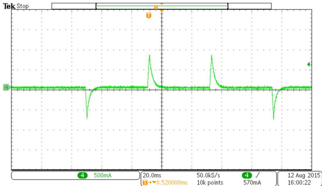
Figure 37. Motor Phase Current With 24-Hz IPD Clock
