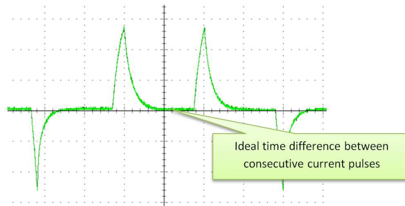
Figure 21. Current Waveform During IPD Process With Optimized 'IPD Clock' Frequency
