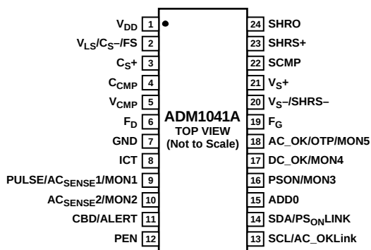
Figure 7. Pin Configuration
